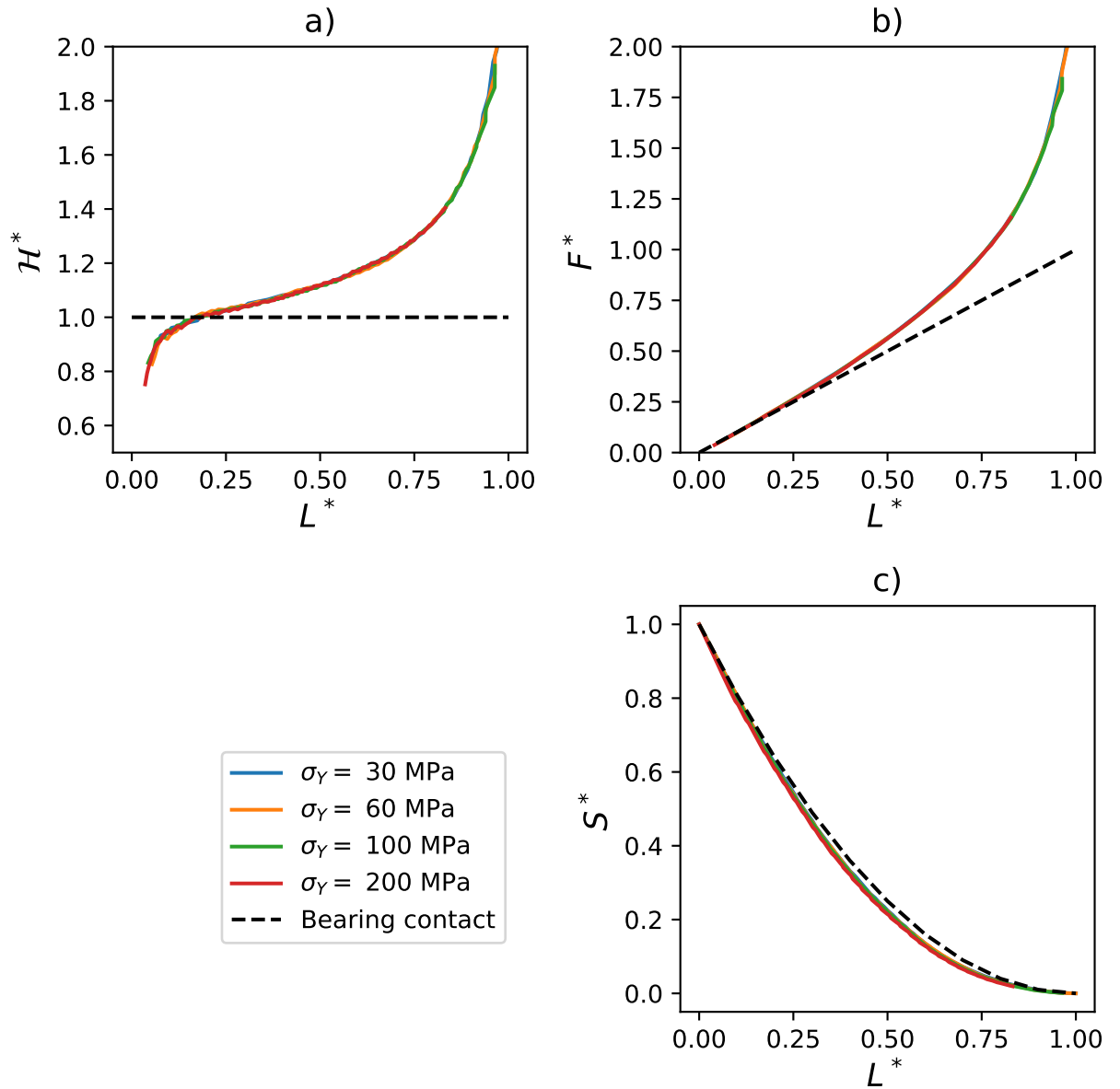
Figure 13: Influence of the yield stress on the multiple wedges indentation, with n = 0.2 .
