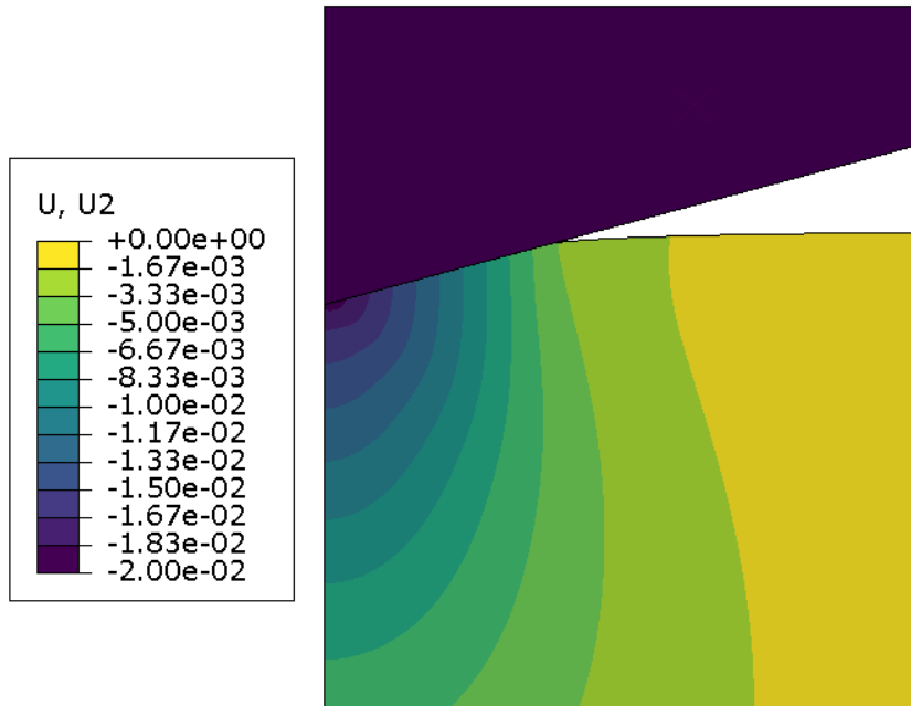
Figure 14: Computed vertical displacement field in single indentation (with n = 0.3 ). Sink-in is observed as the displacement is negative.
