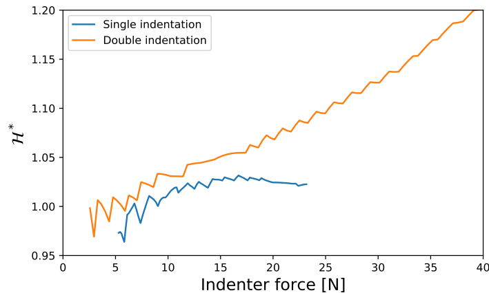
Figure 8: Comparison of the computed instantaneous hardness between single and multiple wedges indentation.
