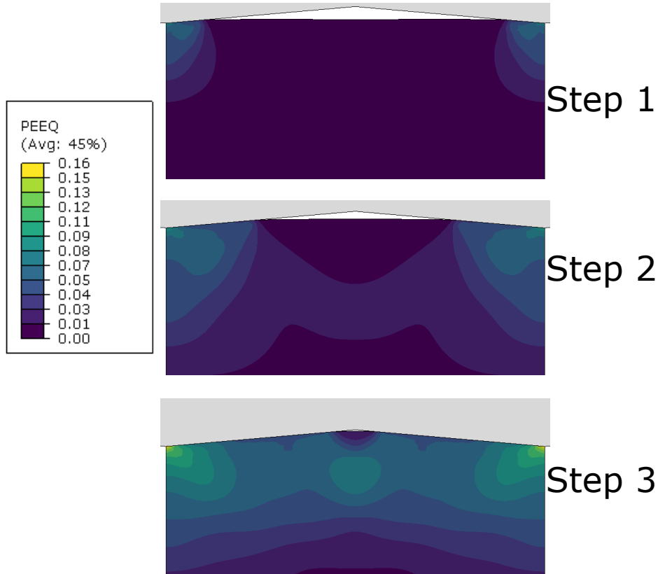
Figure 10: Field of the equivalent plastic strain computed in ABAQUS® for the three stages of the multiple wedges indentation.
