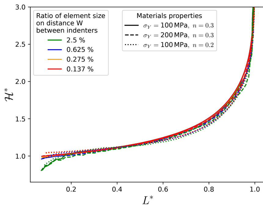
Figure 19: Apparent hardness as a function of the normalized contact area for different mesh size and different materials using an averaging filter
