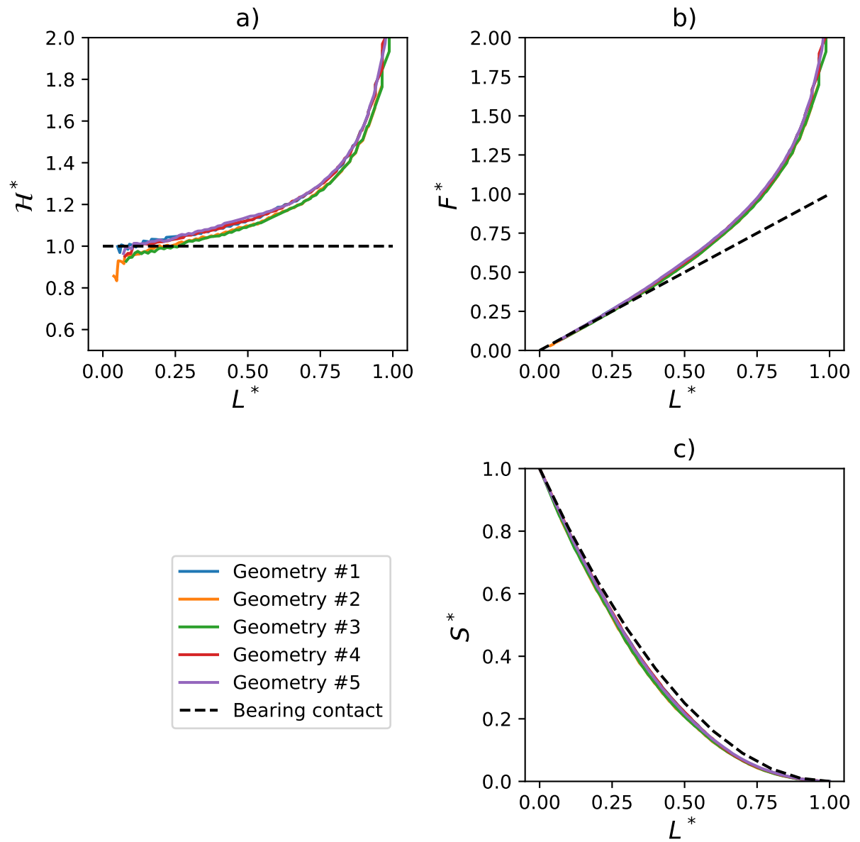
Figure 11: Influence of the geometrical parameters (see Tab. 1) on multiple wedges indentation. The results from the bearing contact model are given as dashed lines.
