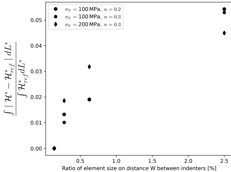
Figure 17: Evolution of the error on the multiple wedges indentation hardness as a function of the relative mesh size, using the most refined mesh as reference.
