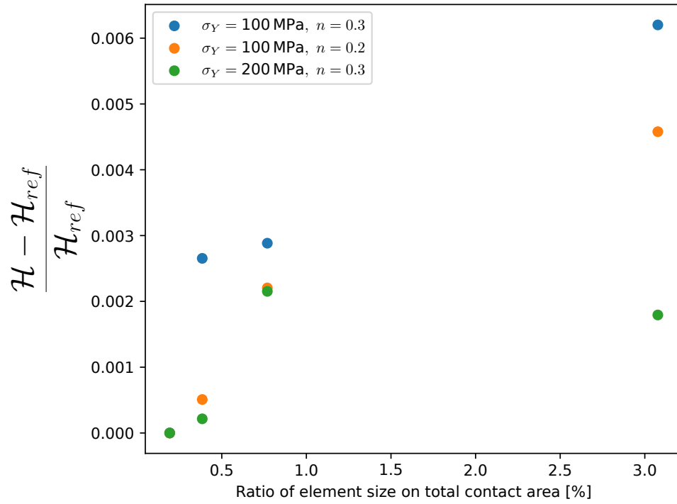
Figure 16: Evolution of the error on the single indentation hardness as a function of the relative mesh size, using the most refined mesh as reference.
