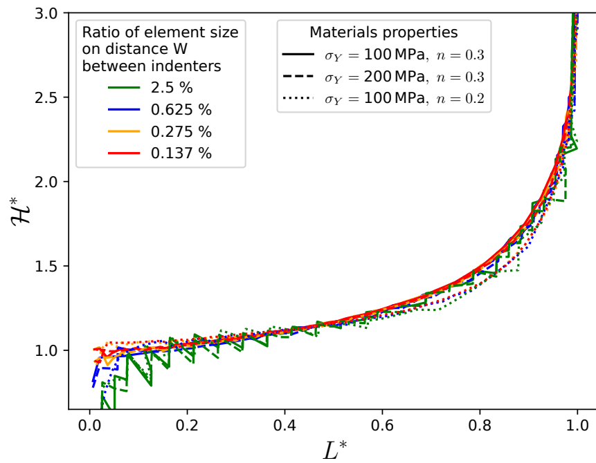
Figure 18: Apparent hardness as a function of the normalized contact area for different mesh size and different materials without averaging filter
