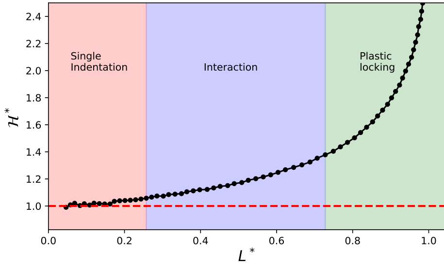
Figure 9: Typical evolution of the hardness as a function of the contact width in multiple wedges indentation, highlighting the three steps.
