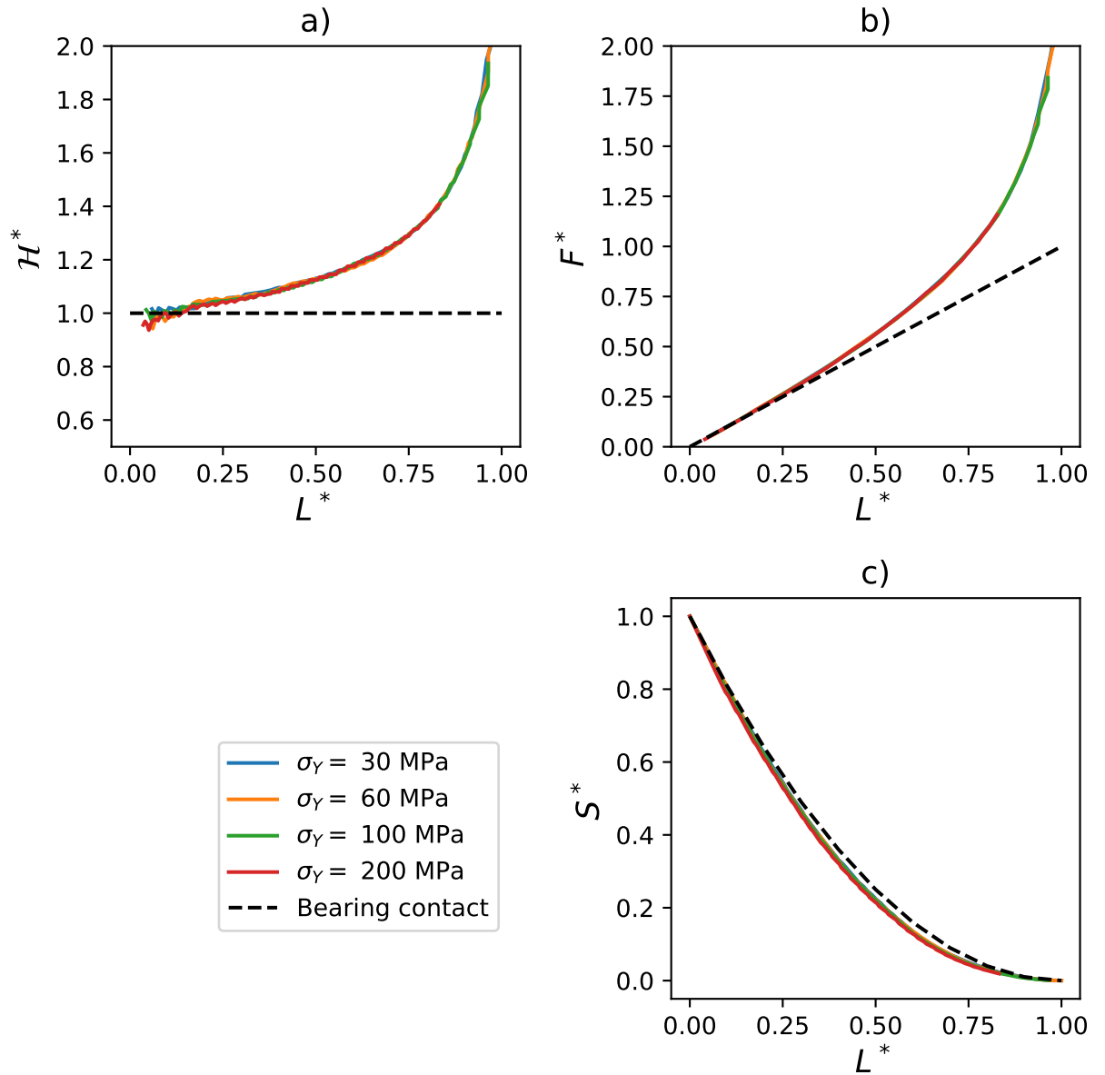
Figure 12: Influence of the yield stress on the multiple wedges indentation, with n = 0.2 .
