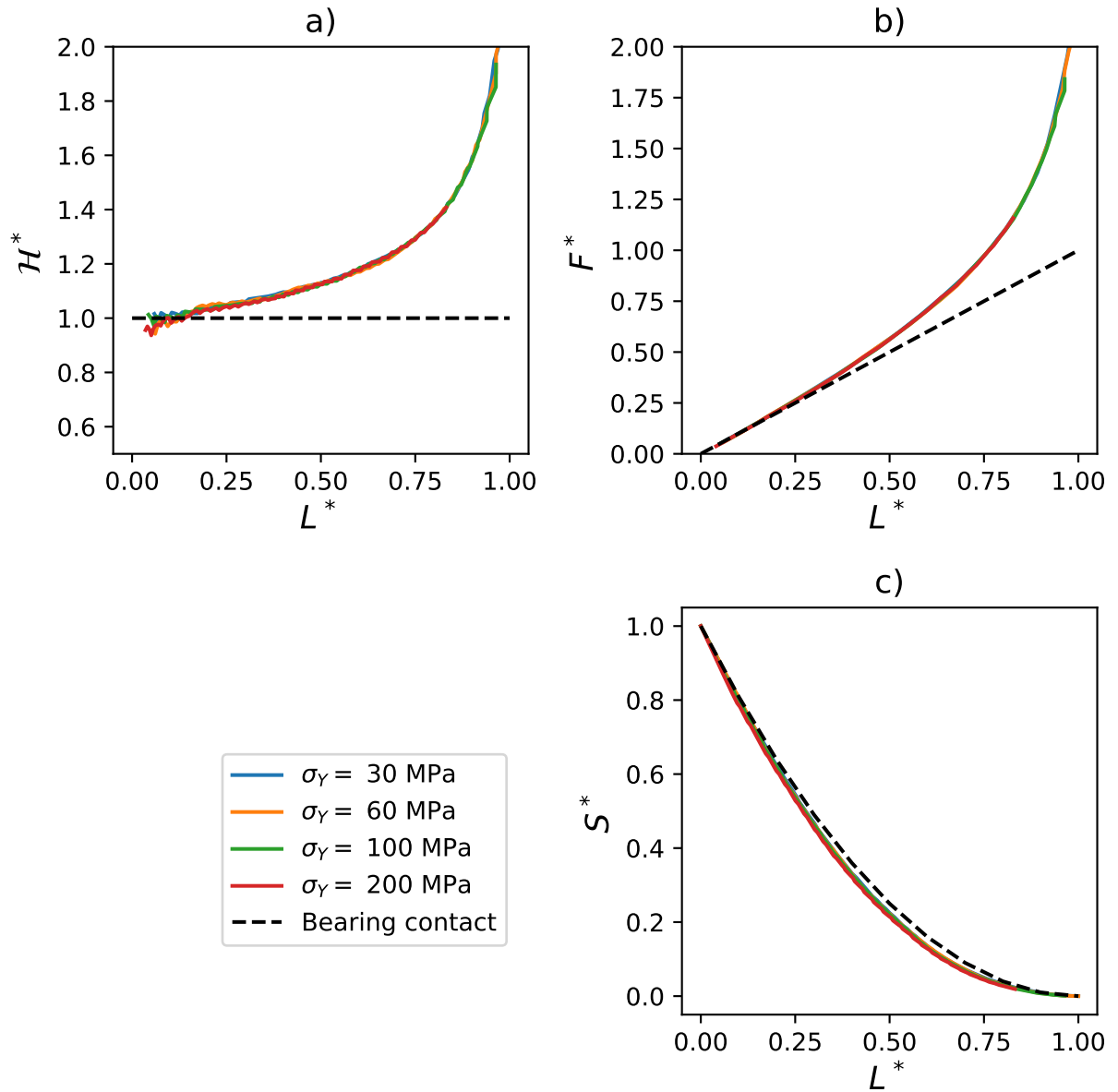
Figure 12: Influence of the yield stress on the multiple wedges indentation, with n = 0.2 .
