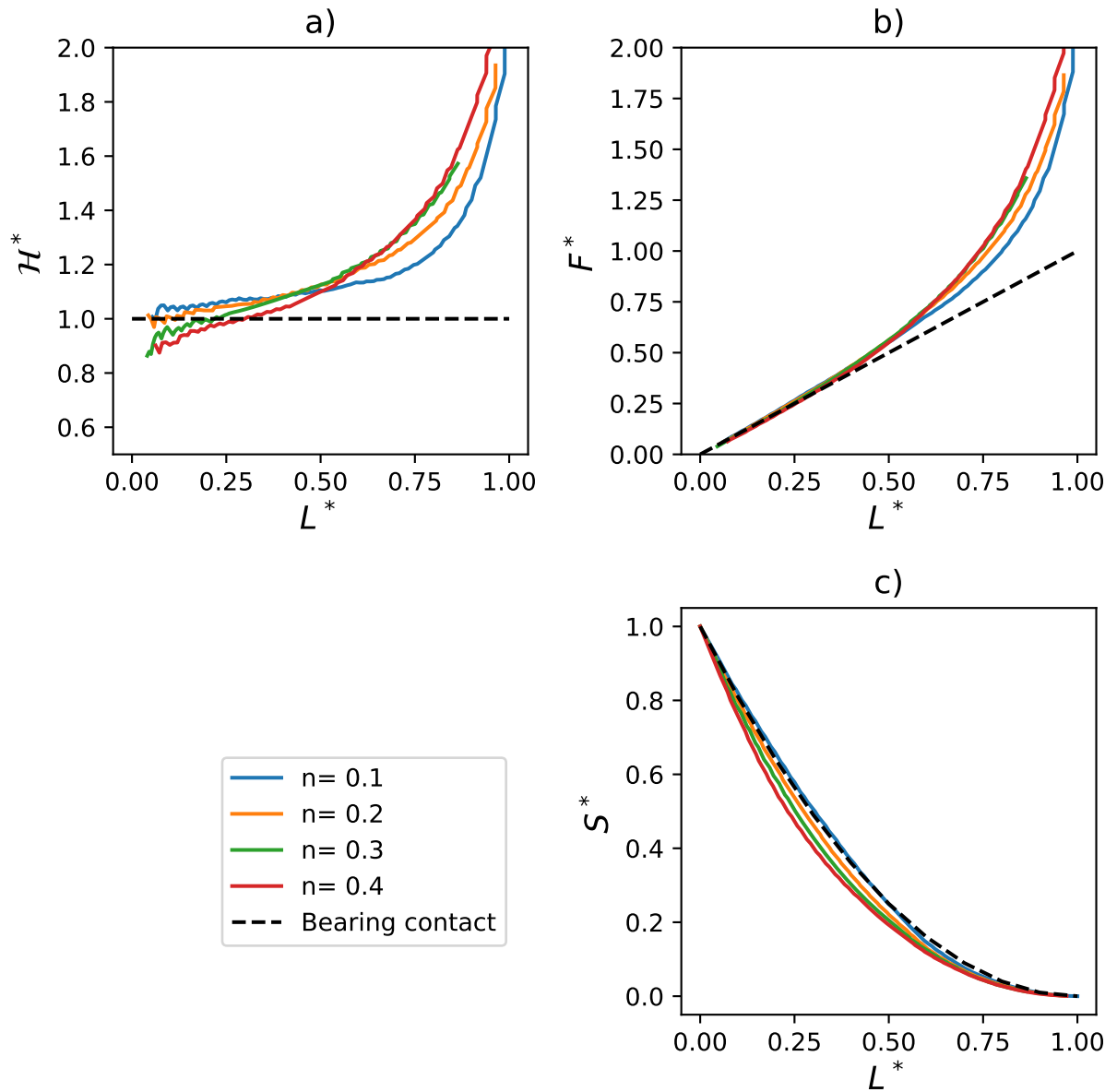
Figure 13: Influence of the strain hardening exponent n on multiple wedges indentation, with \sigma_Y = 100 MPa.
