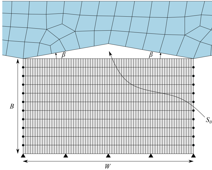
Figure 4: Scheme of the double wedge indentation geometry. The indenter is shown in blue and the substrate in grey.
