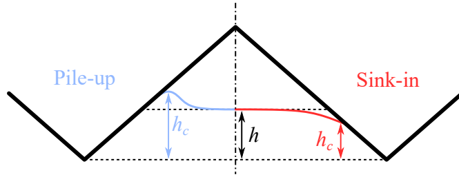
Figure 13: Illustration of the pile-up (blue) and sink-in (red) behaviours of the deformed surface in indentation.
