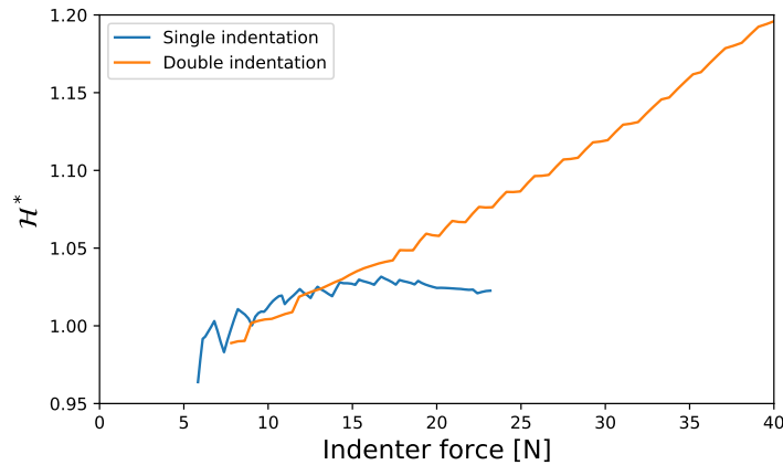
Figure 7: Comparison of the computed instantaneous hardness between single and double wedge indentation.
