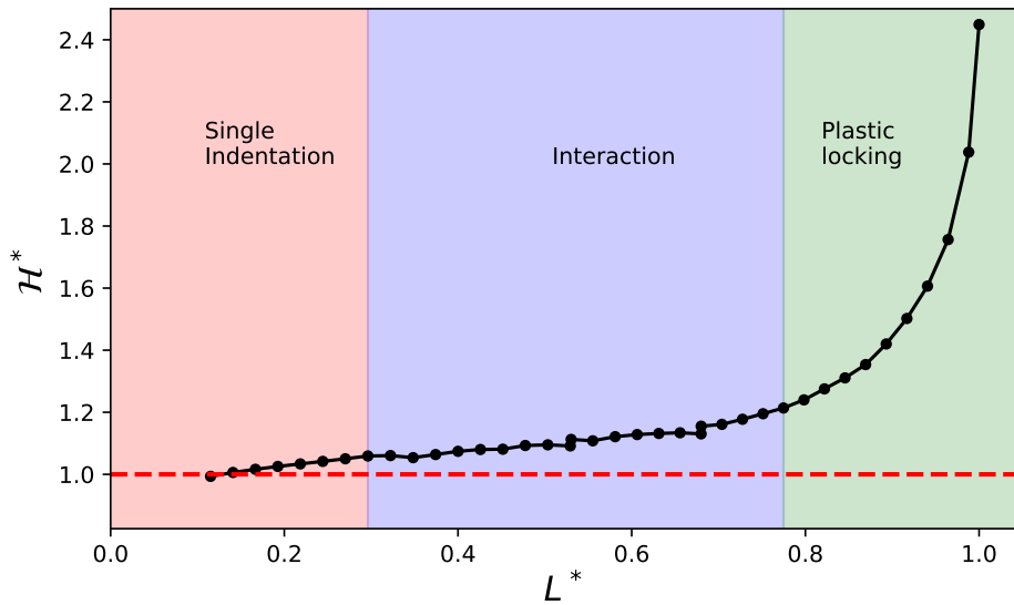
Figure 8: Typical evolution of the hardness as a function of the contact width in double wedge indentation, highlighting the three steps.
