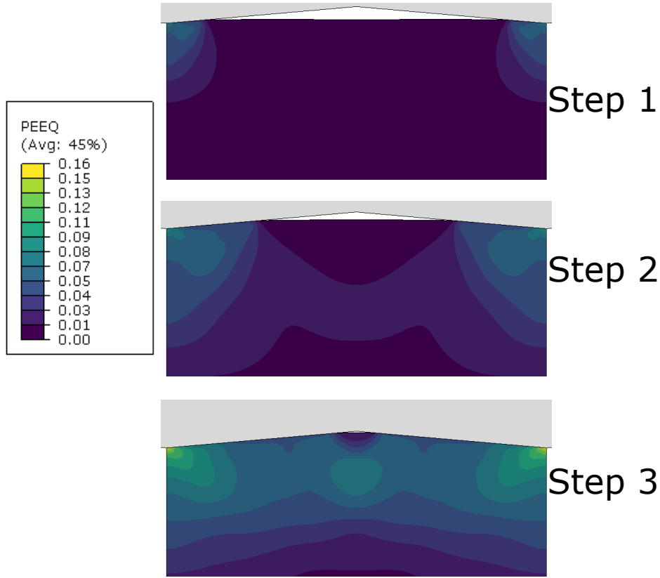
Figure 9: Field of the equivalent plastic strain computed in ABAQUS® for the three stages of the double indentation.
