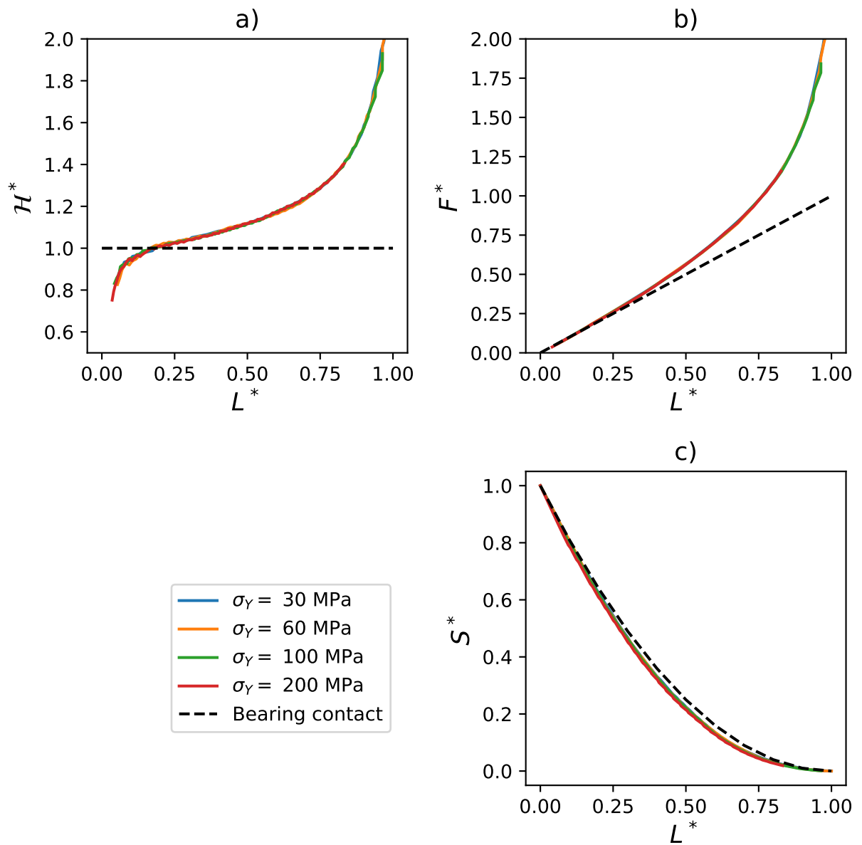
Figure 11: Influence of the yield stress on the double indentation, with n = 0.2 .
