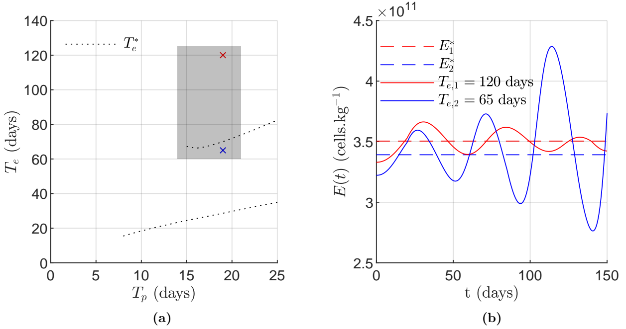
Figure 6 (a) Stability diagram of the improved model associated with the characteristic equation Eq. (22) in the (T_p, T_e) -plane. We remind that T_{e,1} is the parameter used to describe normal conditions, and T_{e,2} a pathological one. A biologically relevant area is colored. (b) Illustrative trajectories associated to example red blood cell transit time specified in (a). The parameters used to obtain these plots are specified in Table 4
