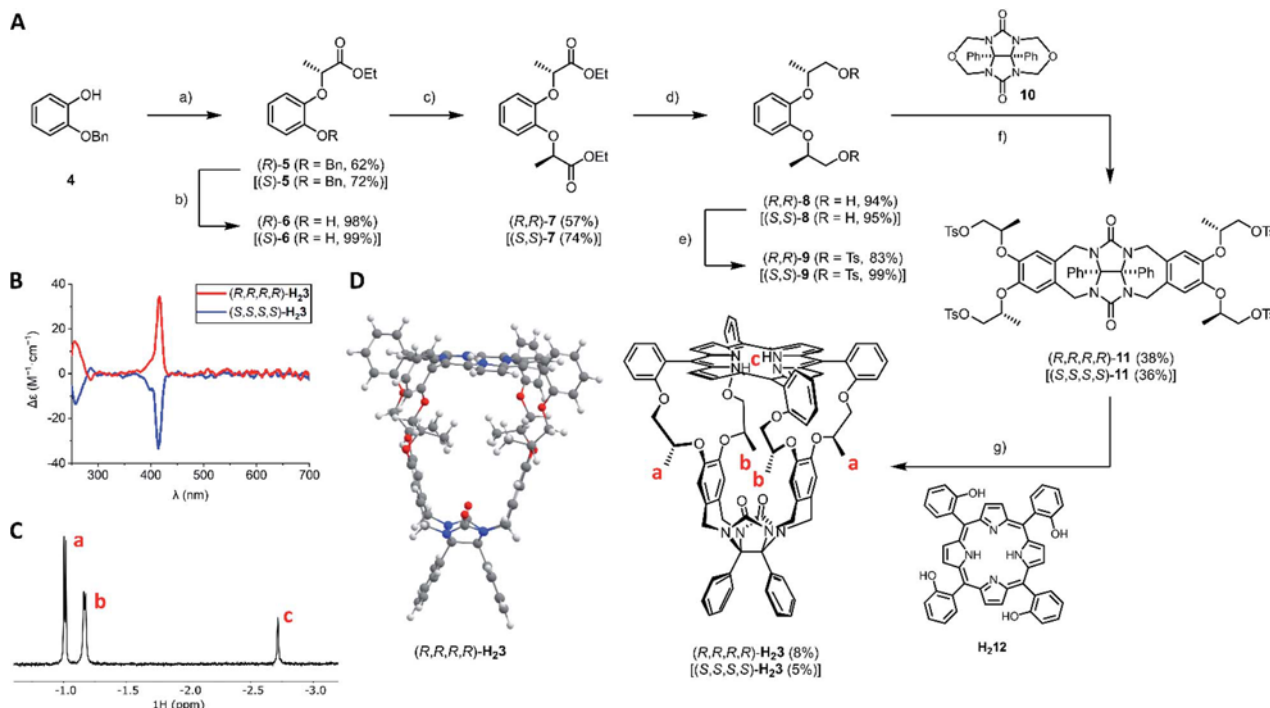
Fig. 2 Synthesis and characterization of H_23 . (A) Synthesis of H_23 ; reagents and conditions: (a) ethyl ( S )-lactate (for ( R,R,R )- H_23 ) or ethyl ( S )-lactate (for ( S,S,S )- H_23 ), DIAD, PPh_3 , toluene, 0 \rightarrow 20^\circ C ; (b) H_2 , Pd/C, EtOAc, 20^\circ C ; (c) ethyl ( S )-lactate (for ( R,R,R )- H_23 ) or ethyl ( R )-lactate (for ( S,S,S )- H_23 ), DIAD, PPh_3 , toluene, 0 \rightarrow 20^\circ C ; (d) LiAlH_4 , THF, 0 \rightarrow 20^\circ C ; (e) TsCl, pyridine, CH_2Cl_2 , 0 \rightarrow 20^\circ C ; (f) ZnCl_2 , SOCl_2 , CH_2Cl_2 , 20^\circ C ; (g) K_2CO_3 , CH_3CN , reflux. For clarity, the synthetic scheme only displays the structures of all ( R )-derivatives; yields of all ( S )-derivatives are indicated in square brackets. (B) ECD spectra of ( R,R,R,R )- H_23 and ( S,S,S,S )- H_23 ( c = 3 \times 10^{-5} M in CHCl_3/CH_3CN , 1 : 1, v/v). (C) Negative chemical shift region of the ^1H NMR spectrum of ( R,R,R,R )- H_23 (400 MHz, c = 10^{-3} M in CDCl_3/CD_3CN , 1 : 1, v/v) with assignment of protons a–c. (D) Front view of the DFT-optimized structure of ( R,R,R,R )- H_23 at the B3LYP/6-311+G(d) level. Color code: white = hydrogen, grey = carbon, blue = nitrogen, red = oxygen.
