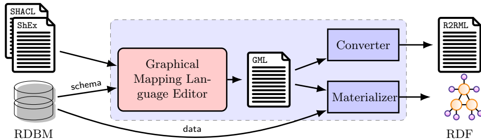
Fig. 2. ShERML Architecture and Workflow.
