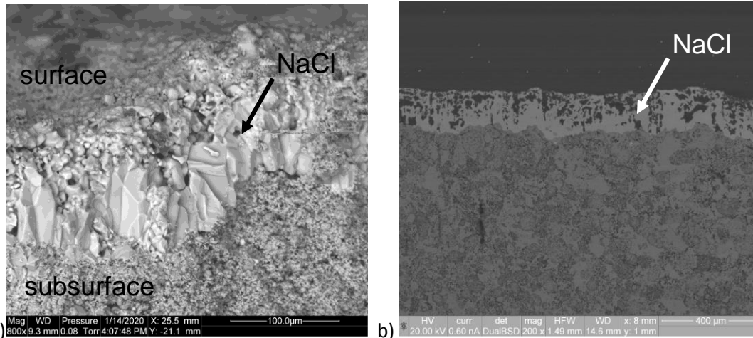
Figure 14: Migné contaminated with NaCl according to procedure P1-1W: (a) SEM image of the ground surface, (b) BSE image of the polished section.
