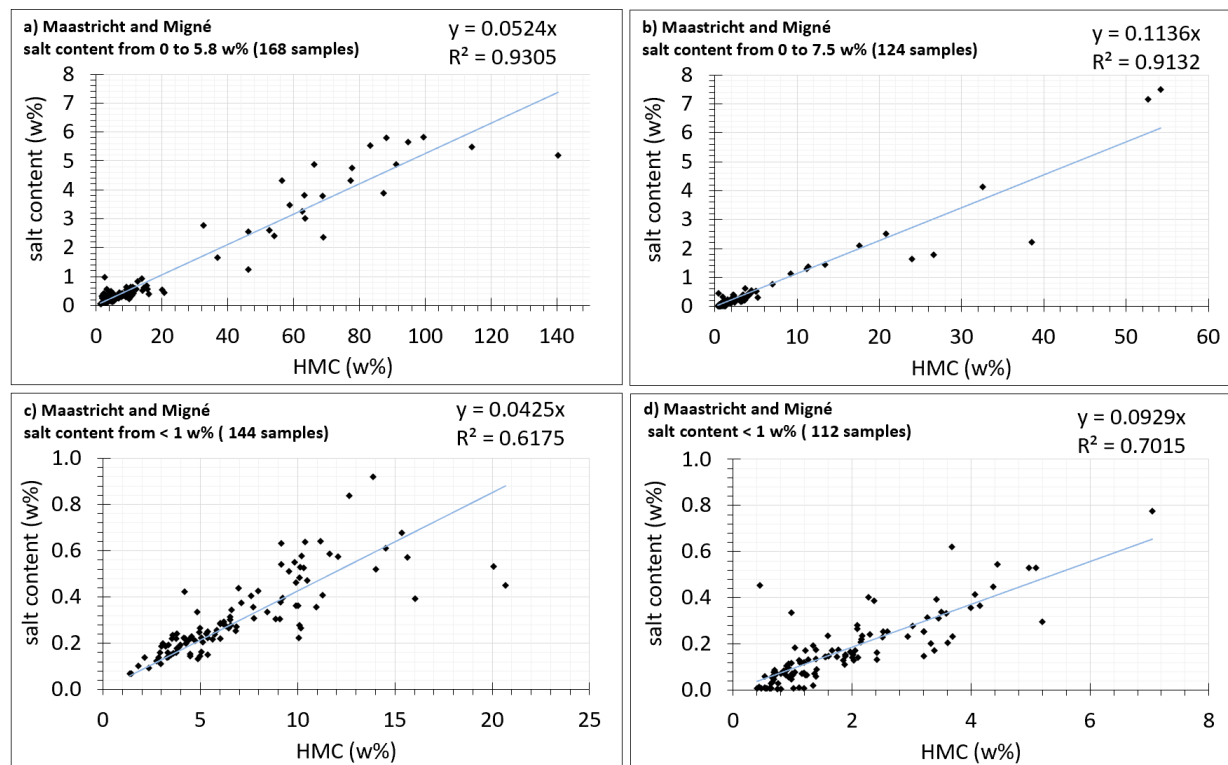
Figure 11: Correlation between HMC values and salt content ( R^2 = coefficient of determination): Maastricht and Migné with NaCl (a) and \text{Na}_2\text{SO}_4 (b) content (full range detected between 0 and 5.8 or 7.5 wt.%) and with NaCl (c) and \text{Na}_2\text{SO}_4 (d) content below 1 wt.%.
