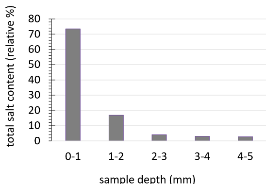
Figure 10: Relative percentage of \text{Na}_2\text{SO}_4 distribution in the first millimetres of Maastricht contaminated with procedure P1-1S.
