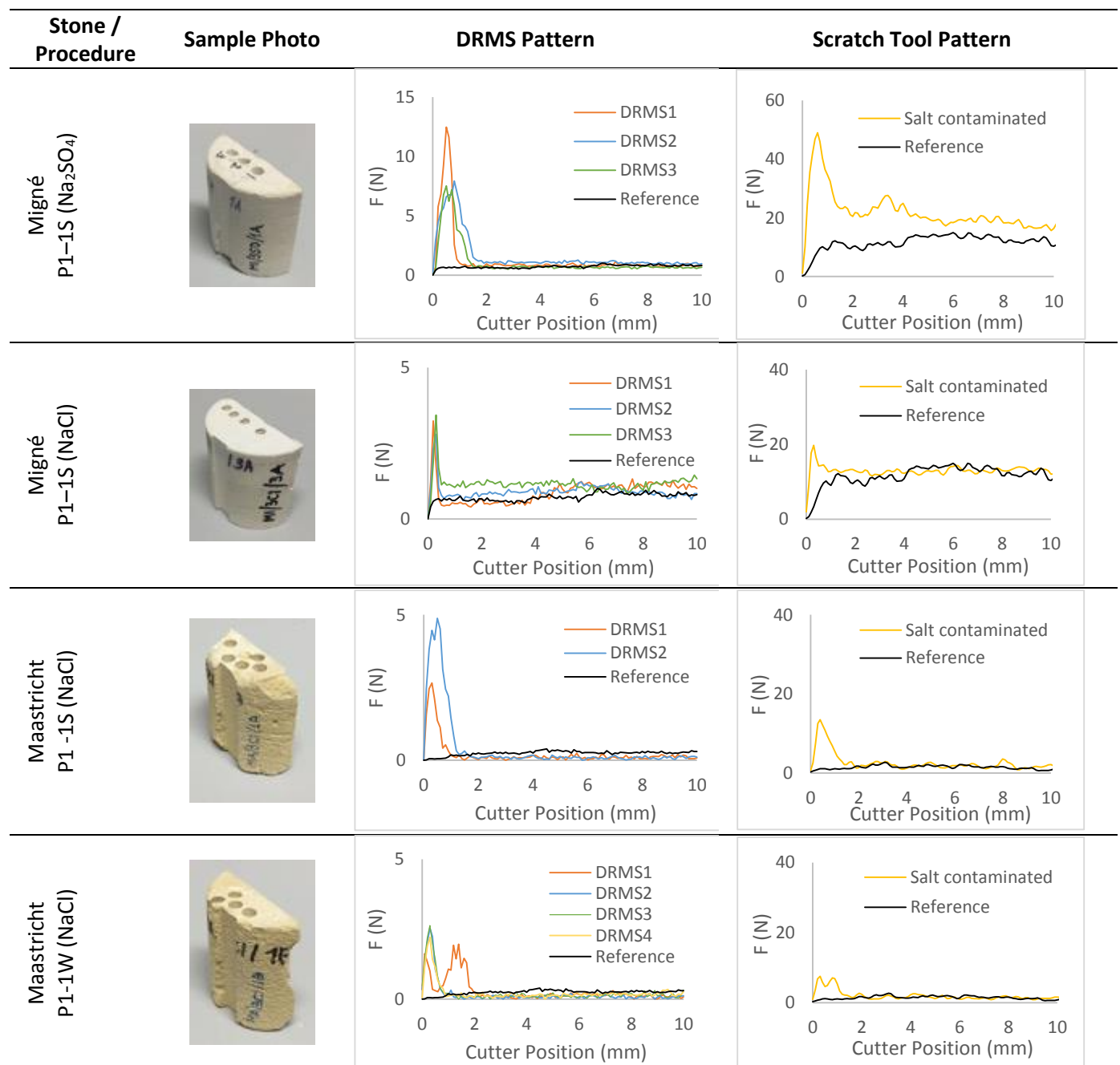
Figure 17: DRMS and average ST patterns for samples contaminated according to procedure P1 (coloured lines) and reference samples (black lines).
