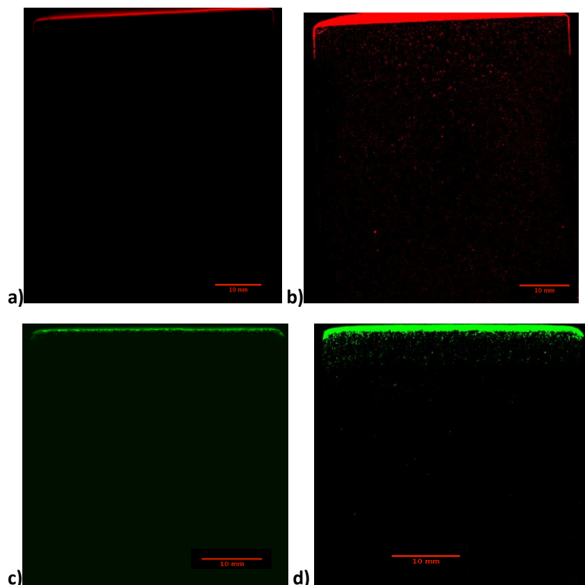
Figure 12: \mu -XRF chloride maps of Migné and Maastricht contaminated according to procedure P1. Migné contaminated according to procedure P1-1S: (a) original map, (b) enhanced map by Image J software; the dense red layer on the top of the sample is an image artefact. Maastricht contaminated according to procedure P1-1W: (c) original map, (d) enhanced map by image J software; the dense green layer on the top of the sample is an image artefact.
