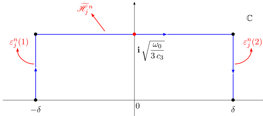
Figure 4: The integration contour in the case \omega_0 \leq \omega \leq 2M . The (approximate) saddle point is represented with a red bullet. The black bullets represent the end points of the three segments along which we compute the integrals
