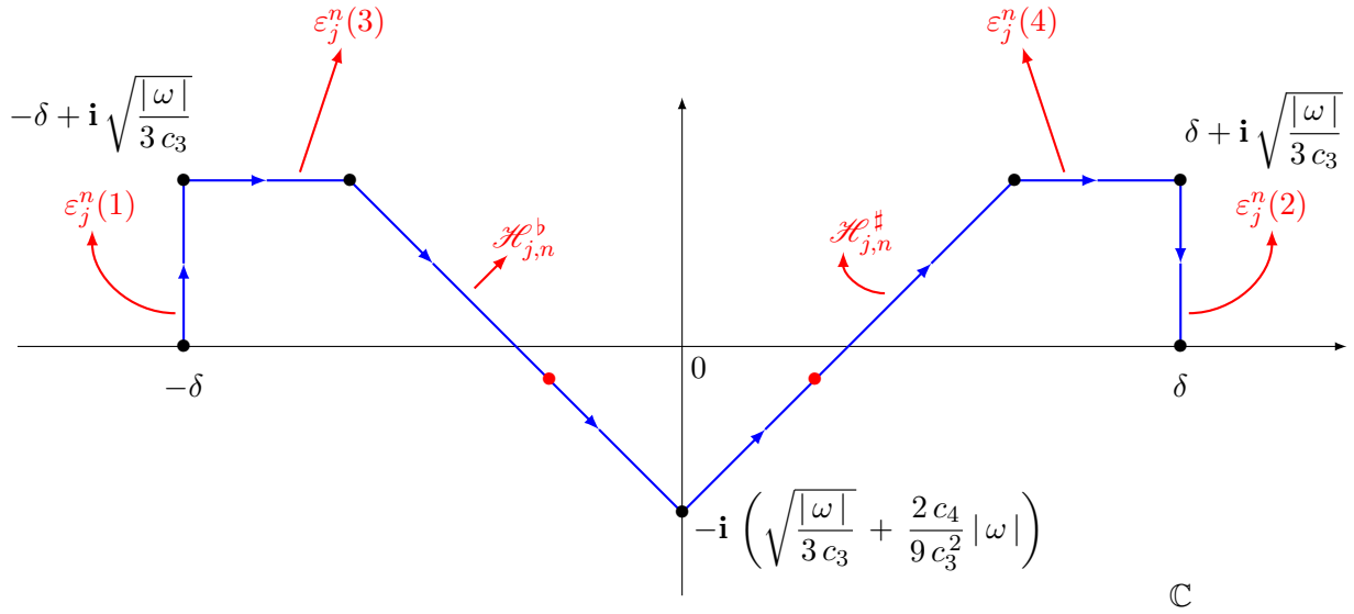
Figure 5: The integration contour in the case -\omega_0 \leq \omega \leq -n^{-2/3} . The two red bullets represent the approximate saddle points and the black bullets represent the end points of the six segments along which we compute the contributions \varepsilon_j^n(1) , \varepsilon_j^n(3) , \mathcal{H}_{j,n}^b , \mathcal{H}_{j,n}^\# , \varepsilon_j^n(4) and \varepsilon_j^n(2) .
