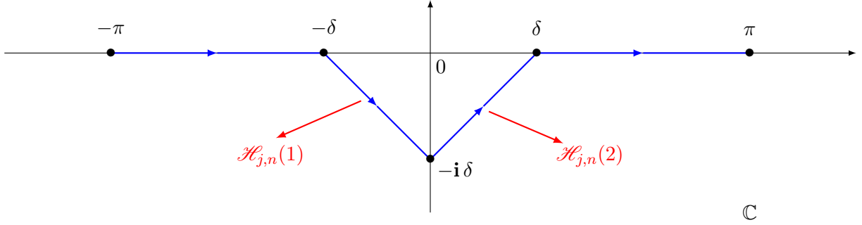
Figure 6: The integration contour in the case -2M \leq \omega \leq -\omega_0 .
