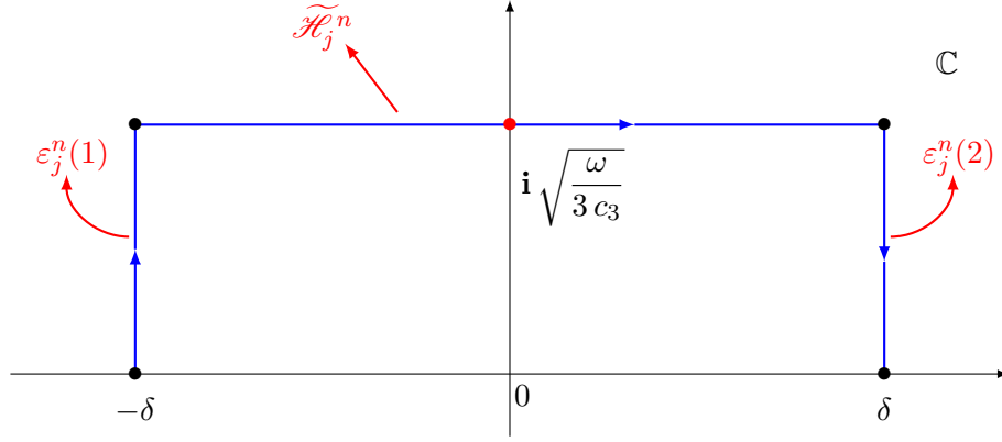
Figure 3: The integration contour in the case n^{-2/3} \leq \omega \leq \omega_0 . The (approximate) saddle point is represented with a red bullet. The black bullets represent the end points of the three segments along which we compute the integrals \varepsilon_j^n(1) , \varepsilon_j^n(2) and \widetilde{\mathcal{H}}_j^n .
