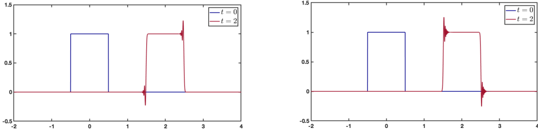
Figure 1: Propagation of a step function by the Lax-Wendroff scheme (2) (left) and Beam-Warming scheme (3) (right) schemes with \lambda = 3/4 . The initial condition is depicted in blue and the numerical solution at time t = 2 is depicted in red.
