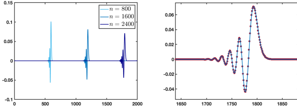
Figure 2: The Green's function of the Lax-Wendroff scheme (2) at various time iterations (left) and a zoom on the oscillations for n = 2400 (right). The chosen parameter is \lambda = 3/4 . On the right: the Green's function \mathcal{G}_j^n in blue and the approximate Green's function \mathcal{H}_j^n defined in (17) in red dots.
