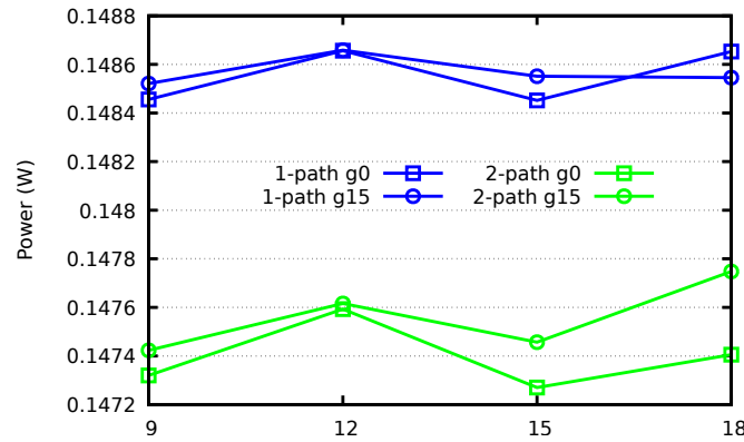
Fig. 9: Mean Power Consumption
