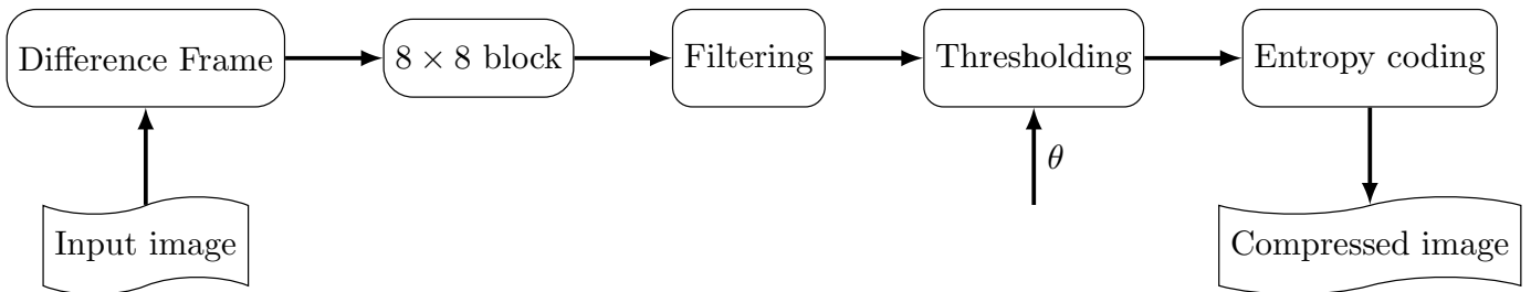
Fig. 3: S-frame encoding sequence
