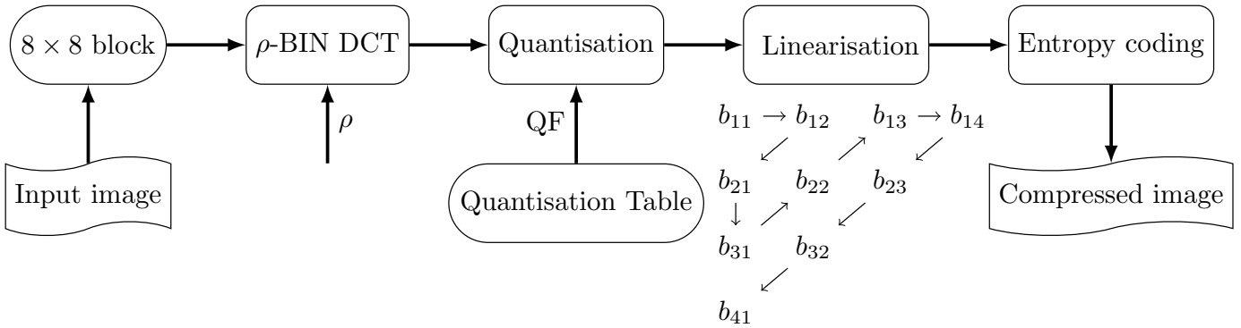
Fig. 2: M-frame block encoding sequence ( \rho = 4 ).
