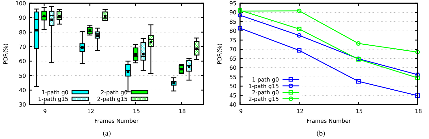
Fig. 6: PDR (a) distribution and (b) mean values
