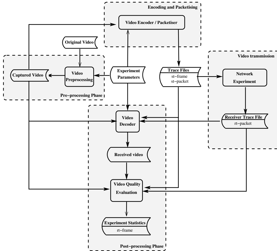
Fig. 5: SenseVid Architecture (redrawn from [Maimour, 2018b])
