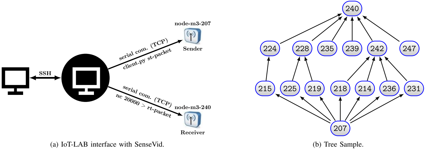
Fig. 4: IoT-lab Experiment Setup
