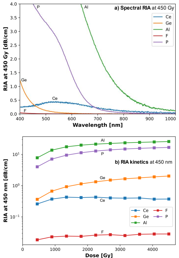
Fig. 9. RIA of all samples. a) Spectral RIA recorded at a TID of 450 Gy. b) Evolution of RIA at 450 nm as a function of TID.
