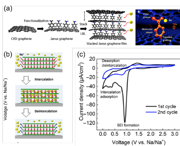
Figure 3. a) Schematic illustration of the preparation of the Janus graphene and the stacked Janus graphene thin film, LbL stands for Layer-by-Layer, b) scheme of the different intercalation/deintercalation cycle of \text{Na}^+ in AB graphene, and c) CV curves measured during the first two cycles of \text{Na}^+ intercalation in AB graphene. The sweep rate was 0.042 mV/s. The first curve shows a sharp cathodic peak, which disappears in the second cycle, corresponding to the formation of a stable solid electrolyte interphase (SEI). Adapted from ref. 12 with permission of Science.
