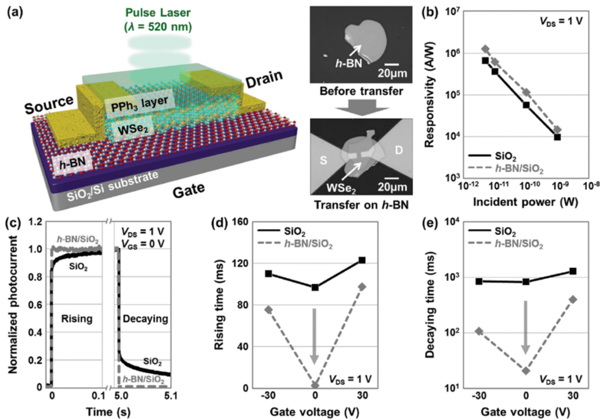
Figure 5. Characterization of \text{PPh}_3 -doped \text{Ti-WSe}_2 / \text{h-BN} photodetectors. a) Schematic diagram and optical images (before and after transfer) of \text{h-BN} inserted into the \text{Ti} -contacted \text{WSe}_2 photodetector that was doped by 7.5 wt% \text{PPh}_3 . b) Extracted photoresponsivity as a function of the incident laser power (5, 10, 100, and 1000 pW) before and after transferring to the \text{h-BN}/\text{SiO}_2 substrate. c) Normalized temporal photoresponse curves at the rising and decaying edges. d, e) Rising d) and decaying e) times of the photodetector as a function of the gate voltage ( V_G = -30, 0, \text{ and } 30 \text{ V} ), where the drain voltage ( V_{\text{DS}} ) was 1 V. Adapted from ref. 20 with permission from Wiley-VHC.
