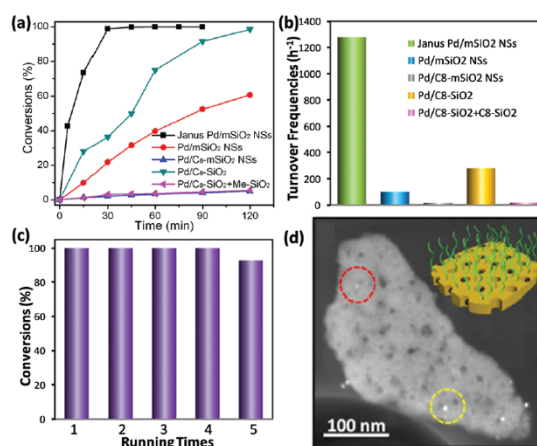
Figure 6. a) The kinetic profile for nitrobenzene reductions over different catalysts under stirring-free conditions. b) Comparison of turnover frequencies (TOFs) for different catalysts. c) Recyclability test of Janus Pd/mSiO 2 nanosheet in biphasic hydrogenation, reaction time: 1.5 h. d) High-angle annular dark-field imaging-scanning transmission electron microscopy (HAADF-STEM) images of Janus catalyst Pd/mSiO 2 nanosheet. Adapted from ref. 35 with permission from The Royal Society of Chemistry
