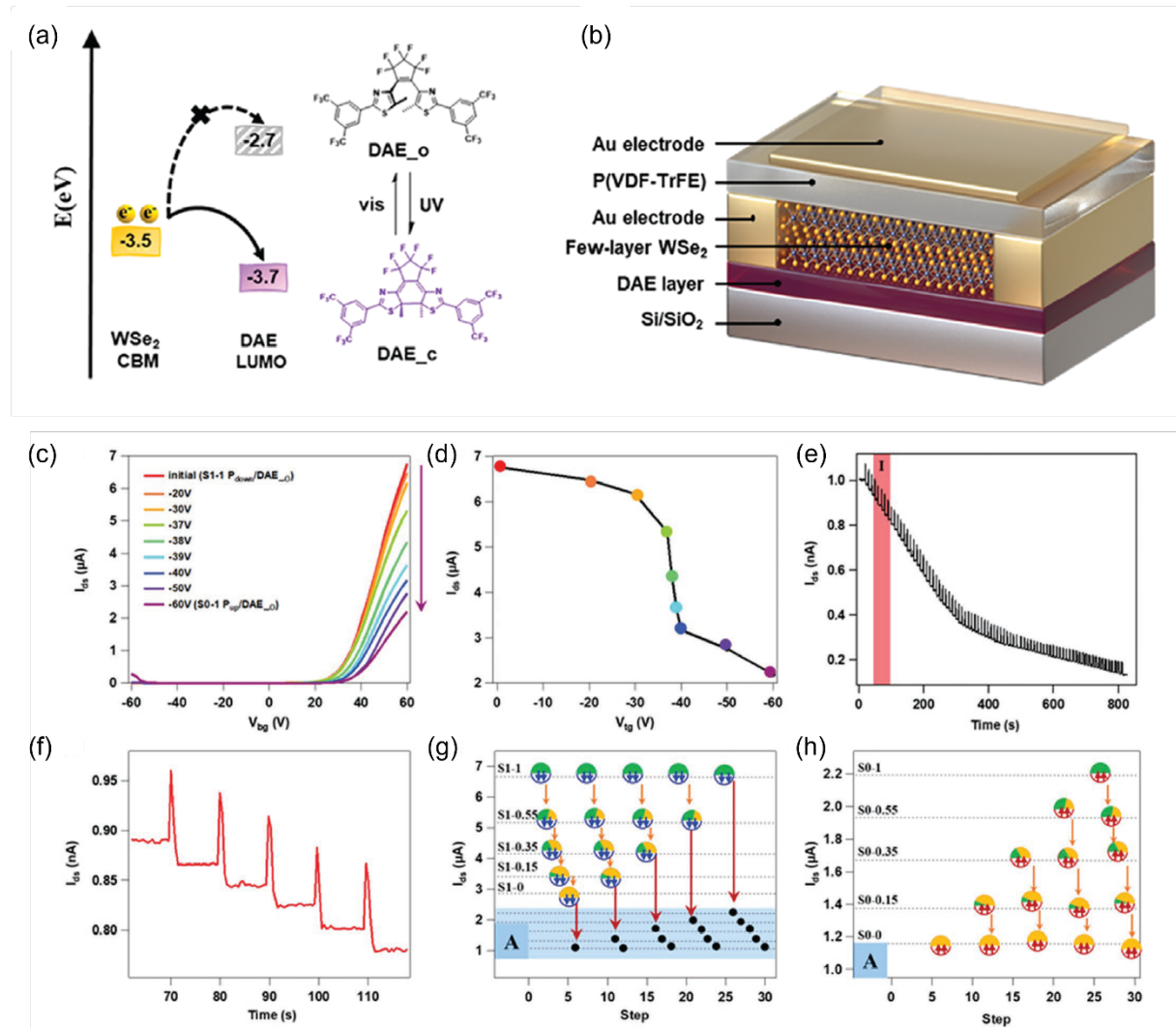
Figure 4. a-b) Energy level diagram between DAE and WSe 2 , device geometry, and electrical characterization of P(VDF-TrFE) capacitor and DAE/WSe 2 /FeFET. a) Energy level diagram of the electron transport between DAE/WSe 2 and the chemical structures of investigated DAE molecules, b) Schematic diagram of the DAE/WSe 2 /FeFET device with double-sided decoration: the bottom surface with DAE film and the top surface with P(VDF-TrFE) layer. c-h) Multilevel storage of DAE/WSe 2 /FeFET. c) Transfer evolution when partially polarizing the P(VDF-TrFE) from downward to upward direction by the sweeping top gate at various ranges. d) Corresponding I ds current evolution
