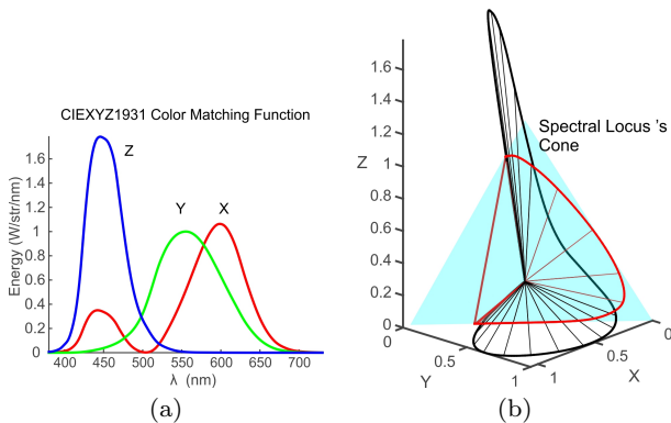
Fig. 2 Cone in CIE color space. (a) Color matching experiment allows to measure three functions of wavelength X , Y and Z . Each value of these functions at a particular wavelength is the amount of intensity of three primaries needed to equalize a monochromatic light at that wavelength. (b) These functions are used to draw the curve of spectrum locus in a three-dimensional XYZ space. In this space the curve (black) is seen as being in the frontier of a deformed cone. This is illustrated by the projection of the spectrum locus on the plane orthogonal to the vector (1,1,1) using the CIE model (red curve).
