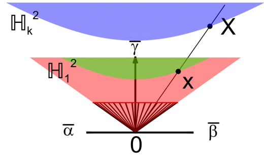
Fig. 13 Projection in Yilmaz-Drösler model. Inside the cone, a natural parametrization is given by a set of hyperboloids of revolution around \bar{\gamma} . Any point \mathbf{X} inside the cone belong to a particular hyperboloid of parameter k = \sqrt{\mathbf{X}^t \mathcal{J} \mathbf{X}} . This point could be projected onto a point \mathbf{x} = \mathbf{X}/(\Sigma k) in the unit hyperboloid. The coordinates (s, \phi) in the unit hyperboloid can be considered as chrominance value whereas the affixe k of X on the line (Ox) is the luminance value of a color.
