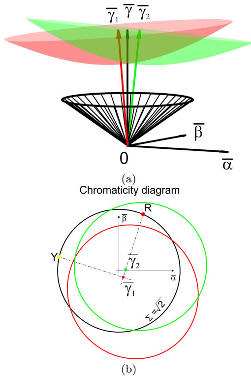
Fig. 15 Transformation from D65 to D50. (a) When the cone is moving with illuminant, the change of metrics corresponds to two different unit hyperboloids centered on each illuminant axis. (b) Representation of the two cones in the chromaticity diagram from the point of view of observer adapted to \bar{\gamma} . The two disks are deformed into ellipses because of the projection in the chromaticity diagram. Yilmaz approximated these ellipses as identical circles (see Figure 6(b)).
