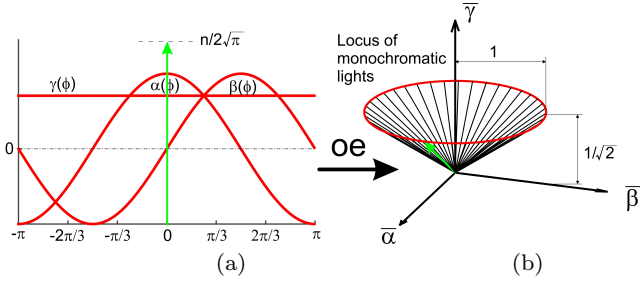
Fig. 12 The cone of perceived color (a) The image of the basis \mathcal{B} of the spectral functions (scaled at n/(2\sqrt{\pi}) ), through the application \alpha , are the vertices of the envelop of the cone materialized by the red circle in (b). Because a light spectral function is a positive function it is a positive linear combination of the vertex, therefore it is located in the interior of the cone. So the image of light spectra is inscribed into the cone C = \alpha(\mathcal{L}^+) . Vertices also correspond to monochromatic lights, thus the envelop of the cone is the image of monochromatic lights which are maximal saturated lights. So the cone envelop is the locus of maximal saturation lights.
