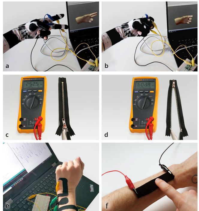
Figure 8. Application examples of polymerization. Cotton gloves capture hand movements (a and b), a zipper is turned into a linear potentiometer (c and d), and kinesio tape becomes a tool for rapidly prototyping on-skin UI’s.
