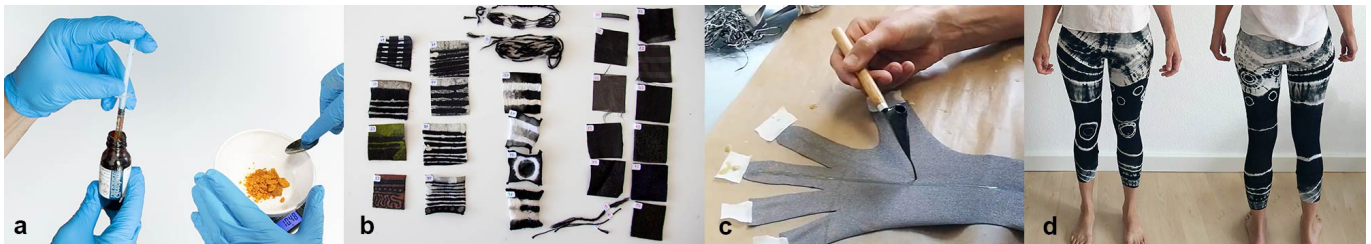
Figure 1. a) Pyrrole (left) and Iron(III) Chloride (right) used for Polymerization. b) Various polymerized samples, of different materials showing tests of batik (left) and tie-dyed traces (middle). c) Traditional manufacturing processes (here Batik) can be used to draw conductive patterns. d) Leggings augmented with polymerization to sense movement.
