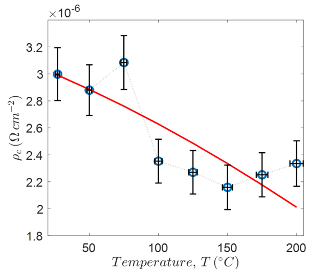
Figure 2. Comparison between experimental specific contact resistivity data (circle) for Ti/Pt/Au (20/30/200 nm) on p-GaAs ( N_d = 1 \times 10^{19} \text{ cm}^{-3} ) extracted from CTLM measurement and model (red line) with respect to the temperature. AuGeNi on p-GaAs was discarded after similar experiment because the specific contact resistance was too high and presents a lower stability to high temperature.
