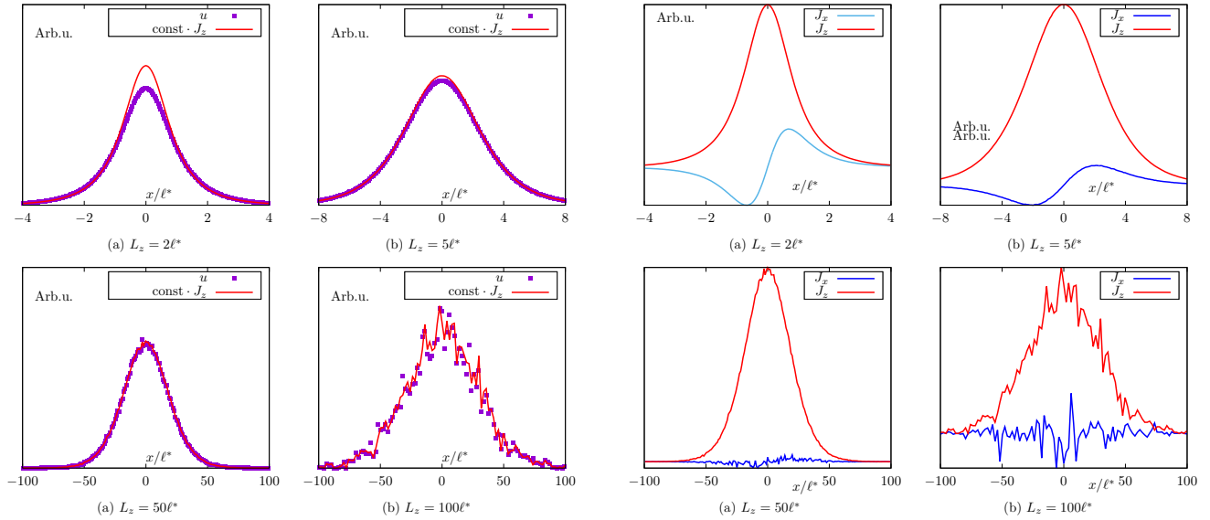
Fig. 1. (left) Comparison of the energy density u(x) and the normal component of the energy current J_z(x) at the exit surface of a slab of the width J_z . The X -axis is parallel to the surface of the slab and intersects with the axis of the incident beam at the point x = 0 . The empirically found constant is \text{const} = 1.7 . The two functions can be made to coincide with good precision (modulo the correct choice of \text{const} ) in the cases L_z = 50\ell^* and L_z = 100\ell^* but not in the cases L_z = 5\ell^* and L_z = 2\ell^* .
