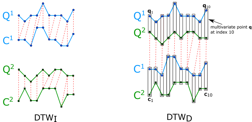
Fig. 1 Independent DTW ( DTW_I , on the left) and dependent DTW ( DTW_D , on the right). Dimension 1 in series Q and C is shown in blue color, and the dimension 2 is shown in green color.
