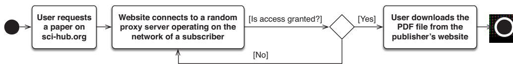
Fig. 9 This activity diagram shows how Sci-Hub serves PDF files of papers through proxy servers operating on the networks of worldwide institutions. The user randomly switches proxy servers until he/she get connected to a proxy entitled to download the PDF of the requested paper.
