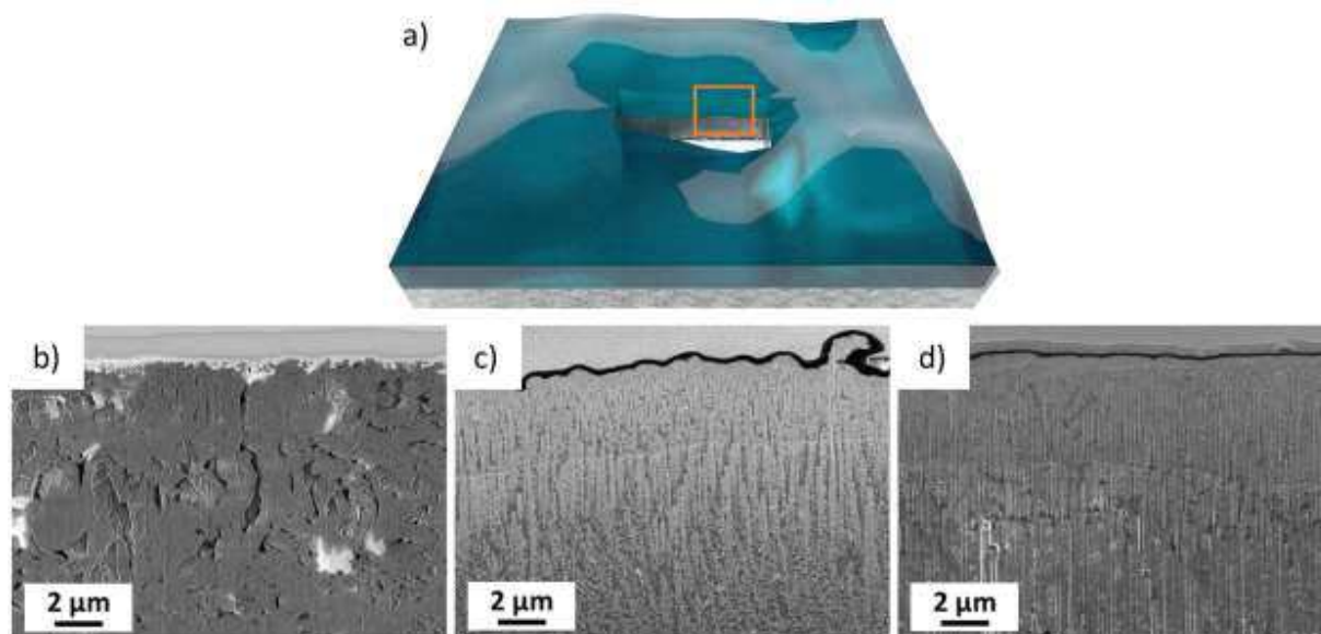
Figure 4. a) Schematic of FIB-SEM cross-sections and FIB-SEM images of b) non-protected lithium after 300 h in classical Li-symmetric cell, c) pristine 0.5% p-TMPETA@Li and d) 0.5% p-TMPETA@Li after 300 h in classical Li-symmetric cell.
