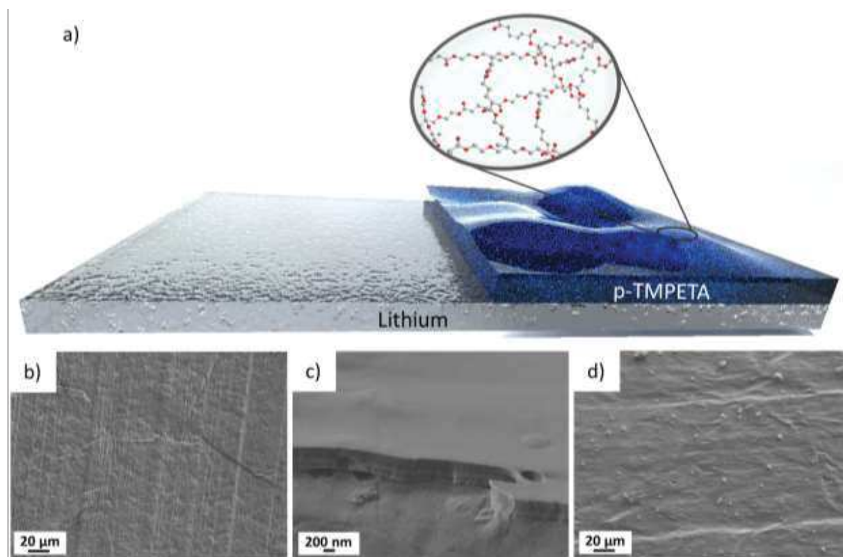
Figure 1. a) Scheme of p-TMPETA on lithium metal surface (p-TMPETA@Li) and corresponding SEM images of the b) pristine non-protected lithium metal c) cross-section of p-TMPETA@Li and d) top-down view of p-TMPETA@Li.
