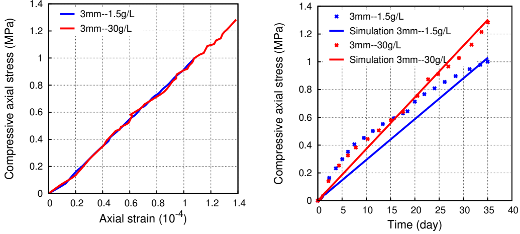
(a) Stress-strain relationship in the axial direction under low-restraint as measured in [50];
