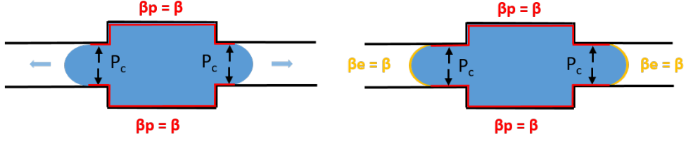
(a) Pore invasion process – Crystals at the crystal-solid interface reach equilibrium \beta_p = \beta by exerting a crystallization pressure according to Eq. 1, namely P_C = \frac{RT}{V_C} \ln(\beta_p) ;
