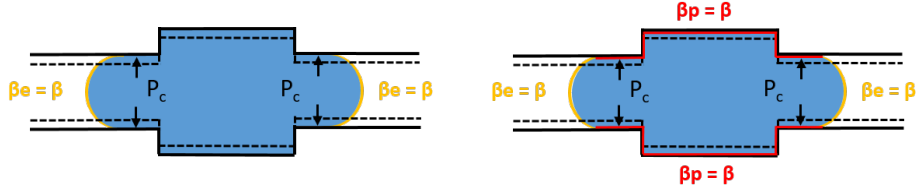
(c) Pore deformation process – Crystals not in equilibrium at the crystal-solid interface but in equilibrium at the crystal-liquid interface \beta_e = \beta ;
