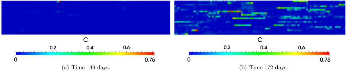
Fig. 6. Uniform and non-uniform C number distribution in the gravitational regime.
