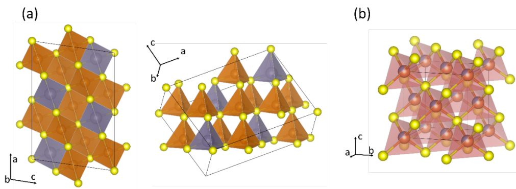
Figure 2. Crystal structure representation of (a) Cu 5 Sn 2 S 7 (space group C2) and (b) Cu 5.133 Sn 1.866 S 6.65 Cl 0.35 (space group F43m). Cu and Sn atoms are shown in orange and grey respectively.
