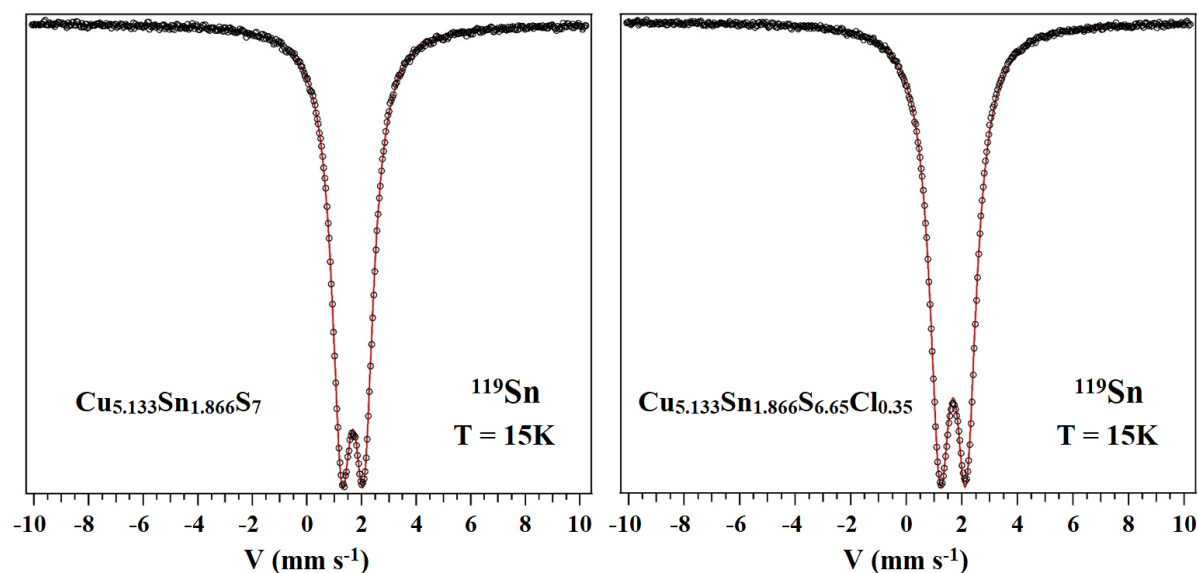
Figure 7. ^{119}\text{Sn} Mössbauer spectra recorded at 15K of the monoclinic sphalerite-derivative Cu 5.133 Sn 1.866 S 7 (space group C2 ) and cubic sphalerite-type Cu 5.133 Sn 1.866 S 6.65 Cl 0.35 (space group F\bar{4}3m ) samples. Experimental data and least-squares fits are represented by black crosses and red lines, respectively.
