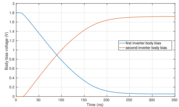
Fig. 6. Body bias voltage convergence for a 28\text{ GHz} input signal with 57.5\% duty cycle
