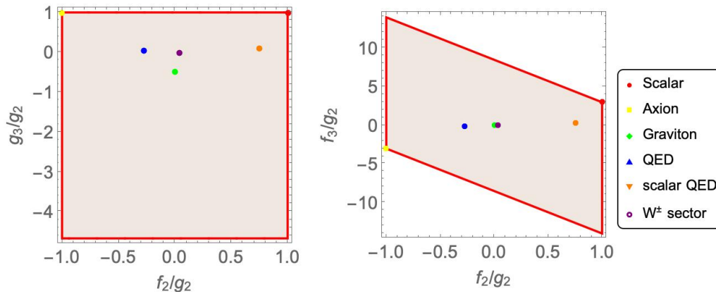
Figure 2: The allowed regions in the \left(\frac{g_3}{g_2}, \frac{f_3}{f_2}\right) vs \frac{f_2}{g_2} space with scalar, axion, graviton, QED, scalar QED, W^\pm sector benchmarked.
