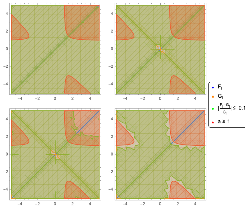
Figure 8: A comparison of the crossing symmetric dispersion for the Photon and Graviton cases which are shown in the first and second rows respectively. We have indicated the regions where F_4, F_5 differ from their dispersive analogues G_4, G_5 by less than 10% in green.
