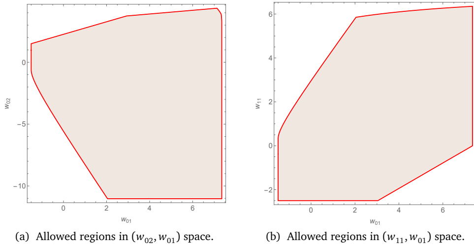
Figure 4: Plots for (w_{11} and w_{02}) vs w_{01} for TR_U^\gamma upto n = 3 .
