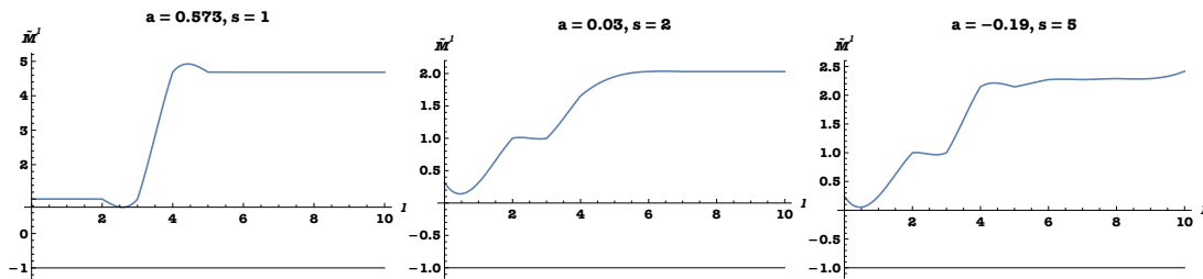
Figure 9: \tilde{\mathcal{M}}^J(s_i, a) vs J for various values of a .
