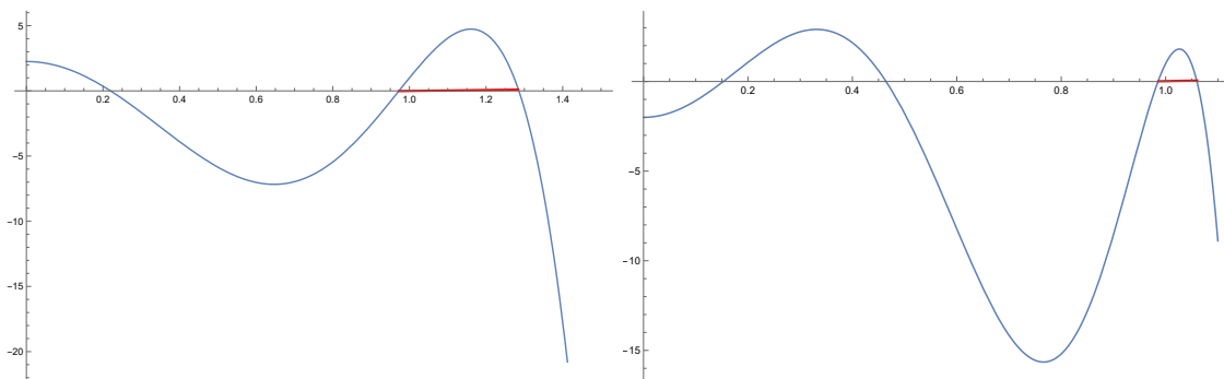
(a) Positive \xi regions for f^{(3)} for J = 9 marked in red. (b) Positive \xi regions for f^{(3)} for J = 11 marked in red.
