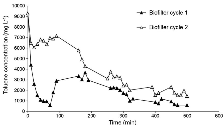
Figure 7. Kinetics of the toluene removal cycles using the biofilter.
