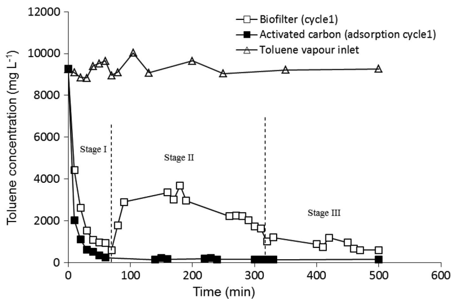
Figure 4. Comparison the performance of biofilter to that of the activated carbon without bacterial attachment towards the removal of toluene vapours inlet.
