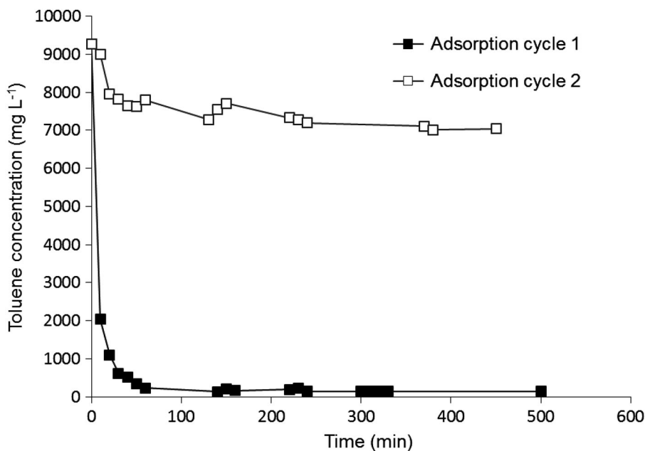
Figure 6. Kinetics of the toluene removal cycles onto virgin activated carbon (without bacteria attachment).
