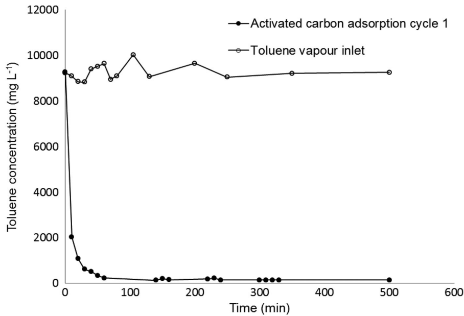
Figure 3. Kinetic adsorption of toluene using activated carbon before Strptomyces griseus DSM-40759 immobilization.
