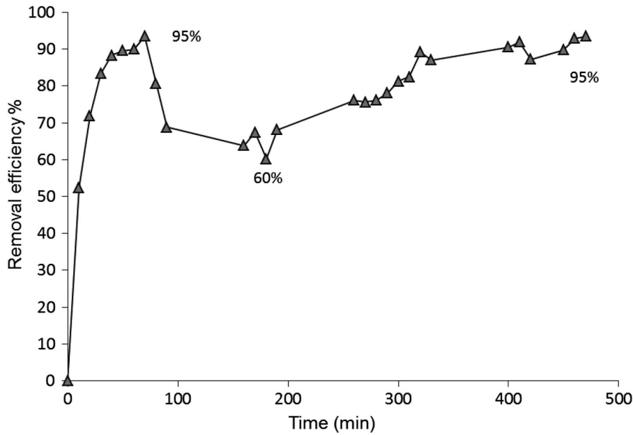
Figure 5. Toluene removal efficiency using the new biofilter.
