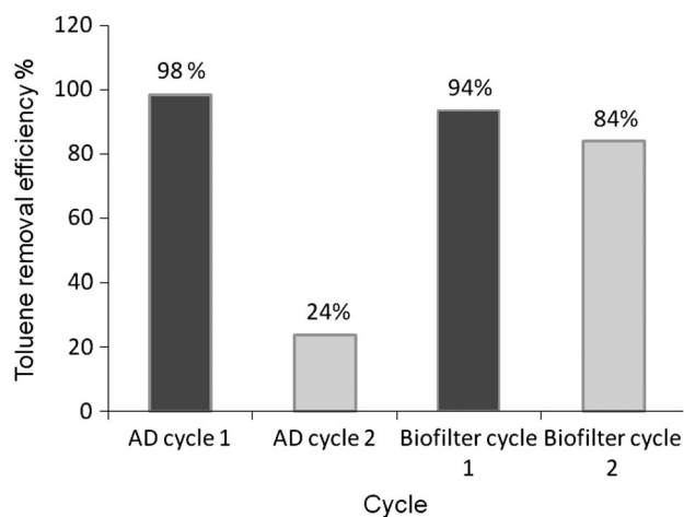
Figure 8. Toluene removal efficiency by using the new biofilter.
