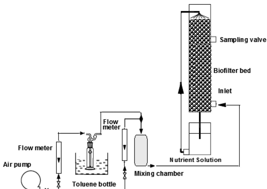
Figure 1. Schematic diagram of the laboratory-scale biofilter system for treatment of air containing toluene.
