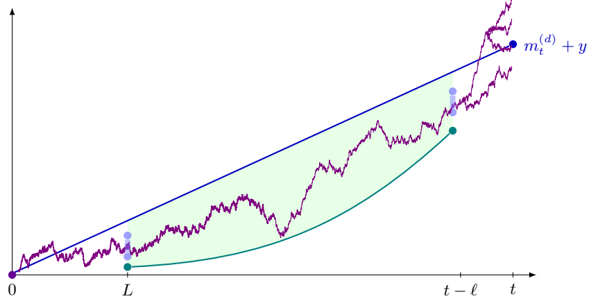
FIGURE 2. Trajectory of the norm of a particle considered in \mathcal{E}_t : at time L are at height in I_L^{\text{in}} , stay in the shaded (green) region up to time t - \ell , at time t - \ell are located in another window, and then produce a descendant that reaches m_t^{(d)} + y at time t .
