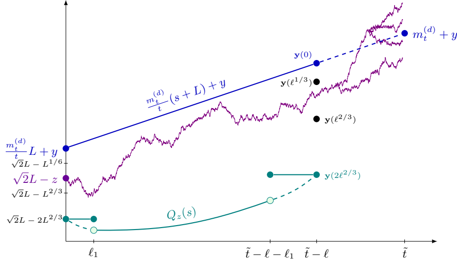
FIGURE 4. The event G_{L,t}(v) \cap \mathfrak{T}(v) from (5.5): the trajectory R^{(v)} of a given particle v \in \mathcal{N}_{\tilde{t}-\ell} is bounded above by the blue line and below by the solid green curves that comprise Q_z on [0, \tilde{t} - \ell] , R_{\tilde{t}-\ell}^{(v)} lies in the window [y(\ell^{2/3}), y(\ell^{1/3})] , and v produces a descendent in \mathcal{N}_{\tilde{t}} that exceeds m_t^{(d)} + y .
