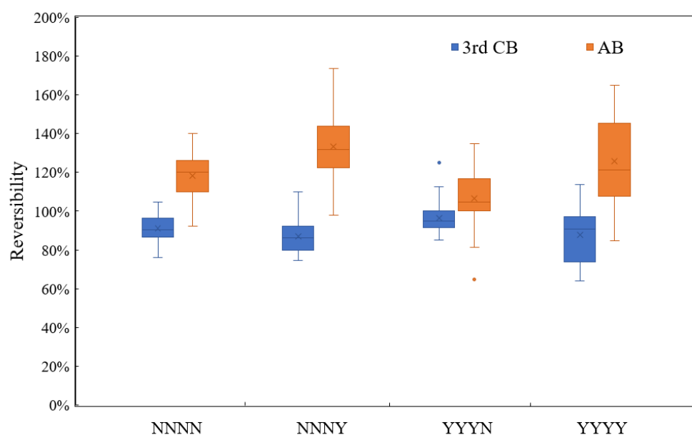
Figure 4. Reversibility ranges of air backwash (AB) and 3rd chemical backwash (CB) in different conditions.
