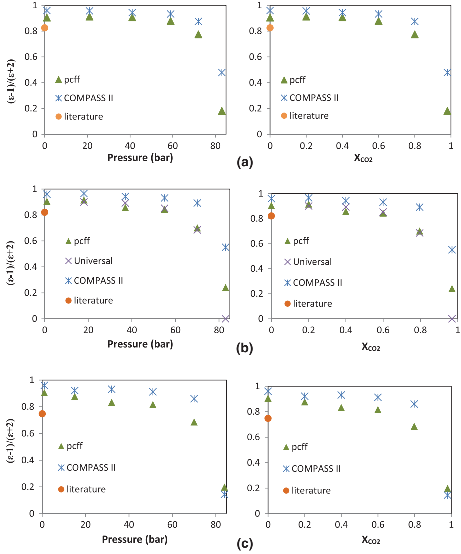
Fig. 10 Reaction field factor (\epsilon - 1)/(\epsilon + 2) of the a \text{CO}_2 /methyl lactate, b \text{CO}_2 /ethyl lactate and c \text{CO}_2 /butyl lactate mixtures at 313 K; the values of \epsilon have been obtained from MD calculations by using different force fields
