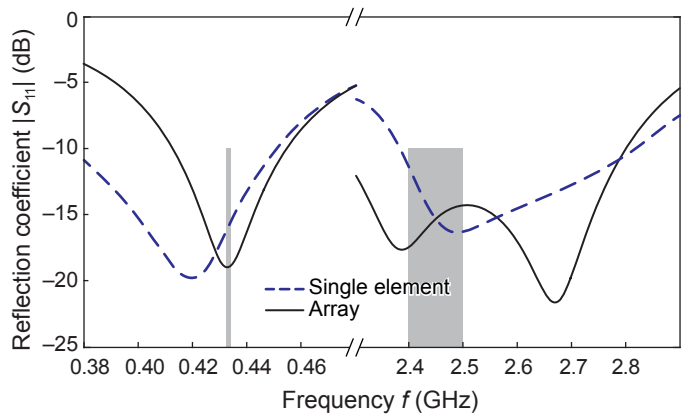
Fig. 4. Comparison of the reflection coefficients |S_{11}| of the antenna in array and single element configurations.
