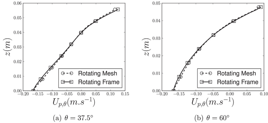
Fig. 12 – Tangential velocity along the z -axis at r=0.08 m and two different angles.
