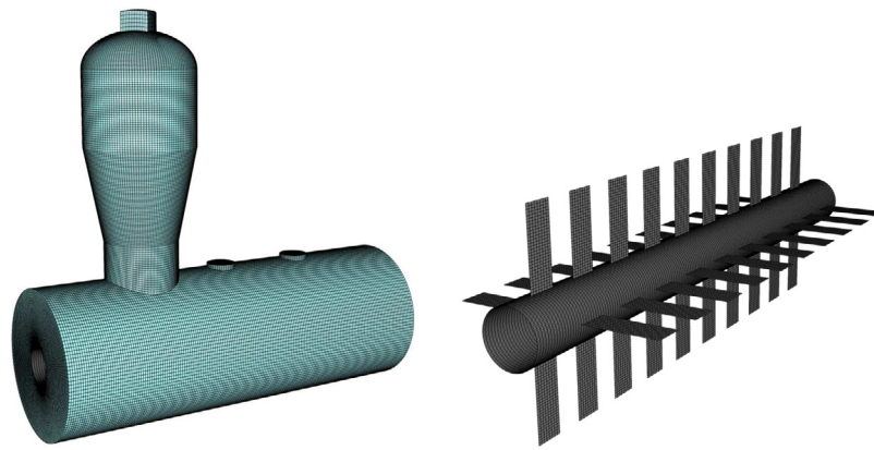
(a) Global view of the mesh (b) The axial stirrer
