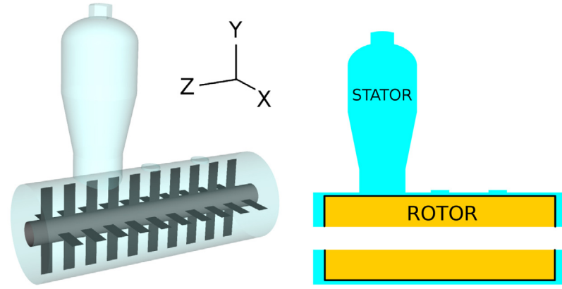
(a) Global view of the reactor and stirrer (b) Rotating and static parts
