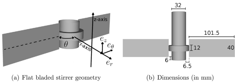
Fig. 9 – Stirrer geometry and dimensions.
