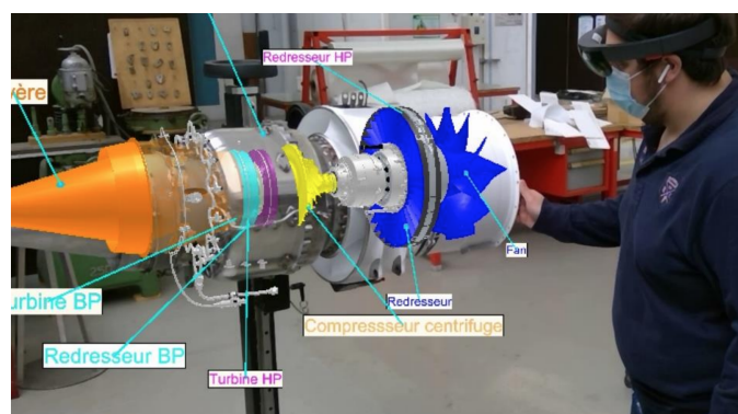
Figure 13. View 01: AR turboprop internal nomenclature with Hololens.
