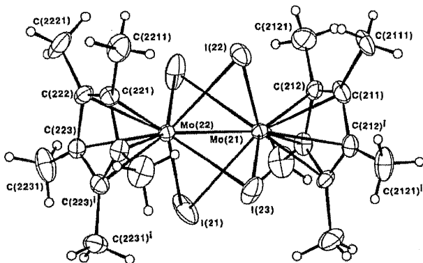
Fig. 1. An ORTEP (Johnson, 1976) view of the [(\eta^5\text{-C}_5\text{Me}_5)_2\text{Mo}_2(\mu\text{-I})_4]^+ cation. Ellipsoids are plotted at the 50% probability level.
