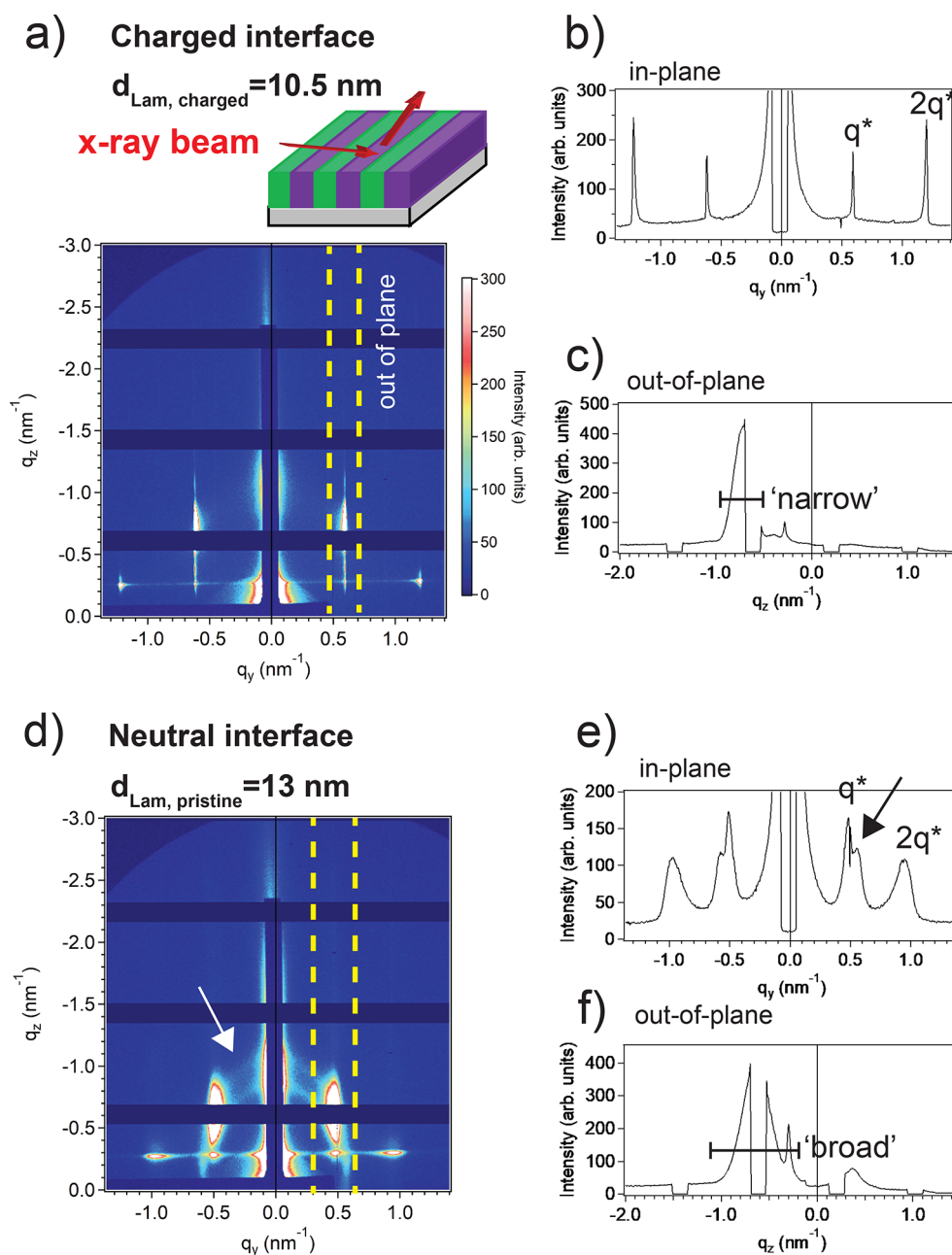
Figure 4. GISAXS results: (a) 2D SAXS pattern recorded for a \text{MH}_{1.2k}(\text{T}^+/\text{TFSI}^-)\text{-PI}_{4.3k}(\text{T}^+/\text{TFSI}^-)\text{-MH}_{1.2k} thin film combined with a scheme showing the X-ray beam configuration with respect to the Lam nanostructure. (b,c) In-plane vs out-of-plane corresponding 1D scattering profiles. (d) 2D SAXS pattern acquired onto a \text{MH}_{1.2k}(\text{T})\text{-PI}_{4.3k}(\text{T})\text{-MH}_{1.2k} thin film. Note that out-of-plane regions are indicated with yellow dashed lines and Debye–Scherrer rings highlighted with a white arrow. (e,f) In-plane vs out-of-plane corresponding 1D scattering profiles.
