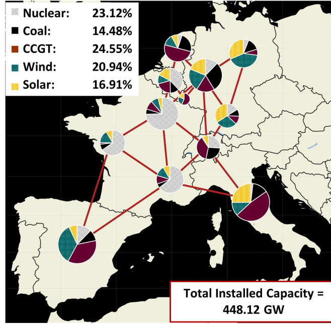
Figure 8: Breakdown of generation capacity per technology and their distribution in the power system before expansion.
