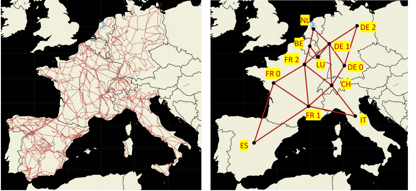
(a) Full power network for the set of European countries selected. (b) Equivalent power system after applying clustering to calculate an equivalent reduced number of buses and transmission lines.
