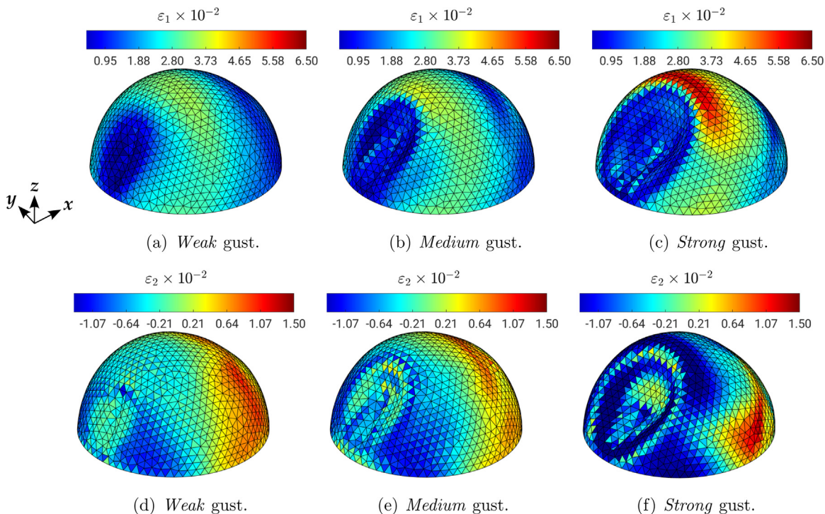
Fig. 19. Flexible FEM case: Distribution of the principal strain values \epsilon_1 ((a) to (c)) and \epsilon_2 ((d) to (f)) for the maximally deflected structure at different gust strengths.
