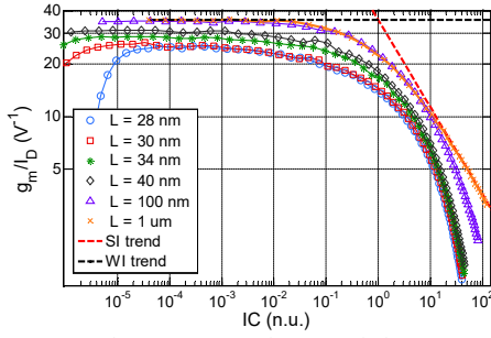
Fig. 7 g_m over I_D charts versus IC for several short NMOS along with a longer channel ( L = 1 \mu\text{m} ) for comparison.
