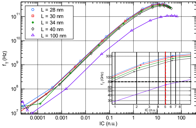
Fig. 4 Measured f_T versus IC for various MOSFET lengths in saturation ( V_{DS}=1V ). Inset gives a focus on the second part of the MI ( 1 < IC < 10 )
