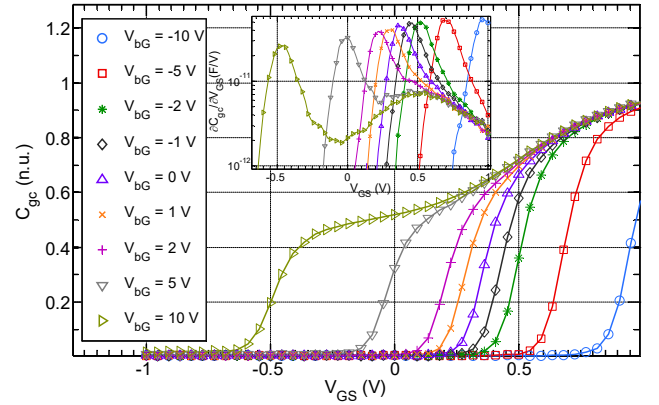
Fig. 2 Measured gate to channel capacitance normalized using front oxide capacitance ( C_{ox}\cdot W\cdot L ) with respect to V_{GS} for various V_{bG} and its derivative (Inset) for N-type UTBB FDSOI MOSFET.
