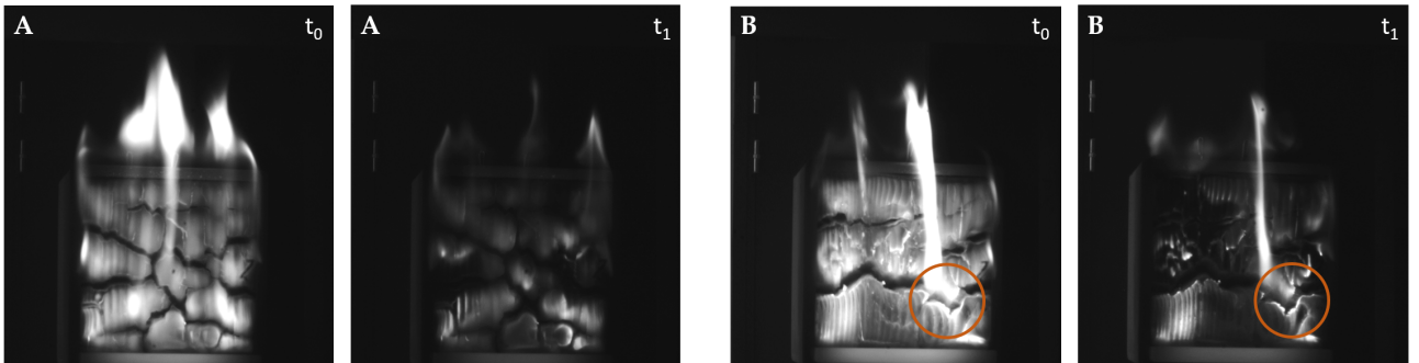
Figure 4: Pictures of two wood samples (A and B) after 15 minutes of exposure to 93.5 \text{ kW}\cdot\text{m}^{-2} . t_0 : time where the heat flux is removed, t_1 : 20 s after t_0 .
