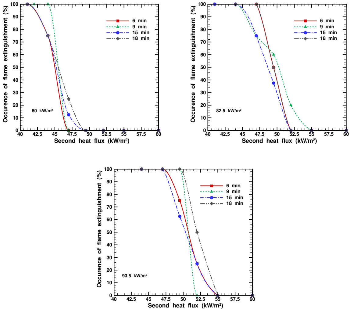
Figure 9: Percentage of flame extinguishment as a function of the heat flux applied to the sample during the second step, for different exposure heat fluxes and different exposure times.
