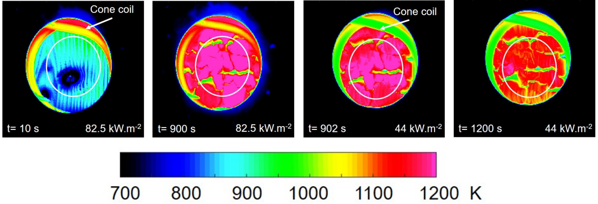
Figure 3: Temperature field in Kelvin and studied area (white circle) at different exposure time for two different external heat fluxes ( 82.5 \text{ kW.m}^{-2} up to 900 s and 44 \text{ kW.m}^{-2} from 902 s to 1200 s).
