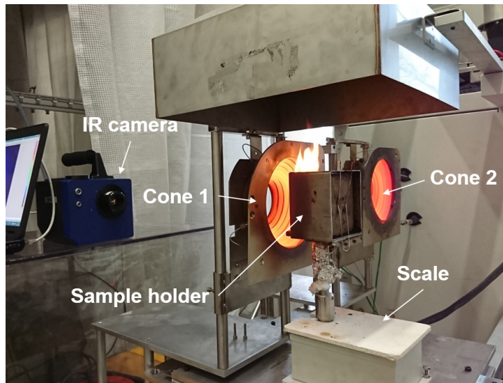
Figure 1: Experimental setup with a flaming wood sample exposed to 82.5 \text{ kW.m}^{-2} (coming from cone 1). Cone 2 is adjusted to a lower heat flux (here 60 \text{ kW.m}^{-2} ).
