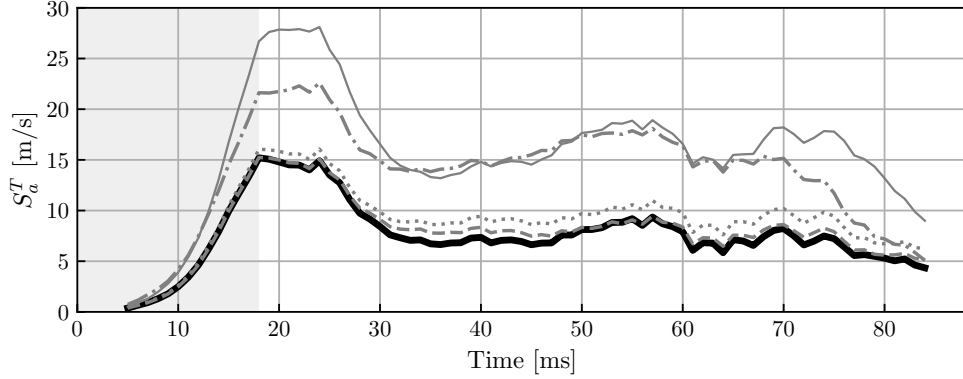
Figure 25: Impact of modeling choices: ( — ): S_a^T of baseline case; ( — ): S_a^T for \beta \equiv 0.5 ; ( - · - · ): S_a^T for S_l = S_l^0(\phi_{glob}) ; ( - - - ): S_a^T with Term III set to zero; ( ····· ): S_a^T for nominal density ratio.
