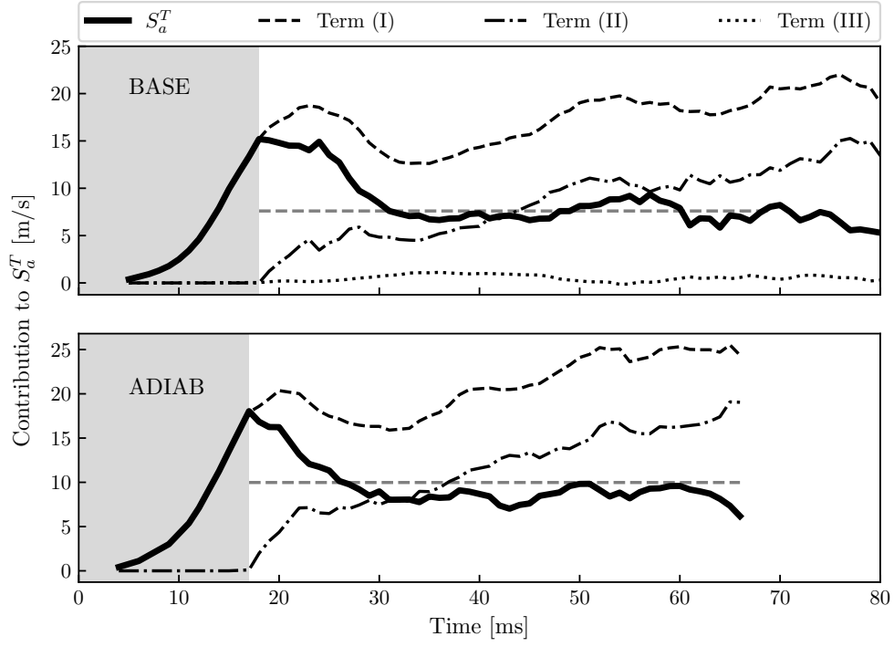
Figure 18: Decomposition of Eq. 15 into three main terms (thin lines) plotted as absolute values for both cases. The absolute turbulent flame speed S_a^T (thick line) is added for reference. The horizontal dashed grey lines correspond to the average velocity obtained from the sector arc length and the averaged elapsed time between two adjacent sector heat release peaks of the respective case (see Fig. 7 for the baseline case).
