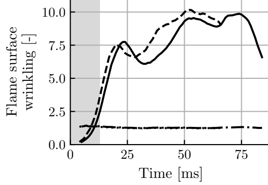
Figure 24: Resolved flame surface wrinkling \Xi_{res} for case BASE (solid line) and ADIAB (dashed line). The sub-grid scale flame surface wrinkling \langle \Xi_{\Delta} \rangle_{res} averaged over the resolved surface is virtually the same for both cases (dash-dotted and dotted lines).
