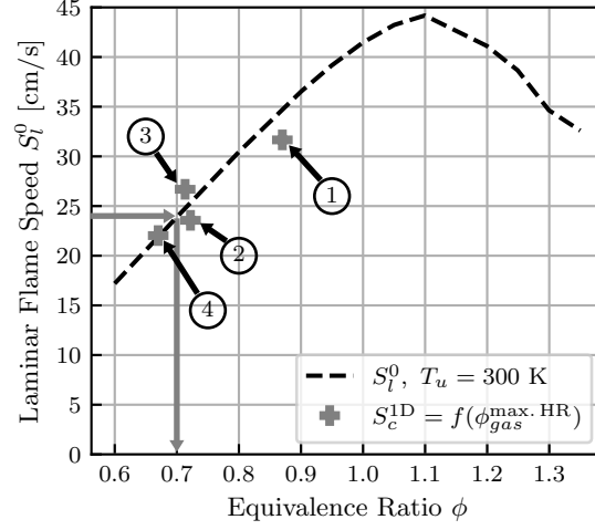
Figure 21: Laminar flame speed diagram for a gaseous n-heptane/air flame at varying equivalence ratios for T_u = 300 K in fresh gases. Dashed line denotes reference data published in [48]. Crosses refer to the one-dimensional laminar consumption speed S_c^\Delta according to Eq. 17, which is computed for arbitrary locations along the flame front indicated in Fig. 19.
