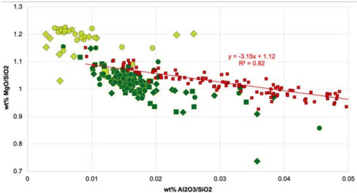
Figure 26: \text{Wt}\% \text{Al}_2\text{O}_3/\text{SiO}_2 vs \text{wt}\% \text{MgO}/\text{SiO}_2 for dunites (light green) and harzburgites (dark green) samples in core from the MBO, compared to estimated and observed compositions of residual mantle lherzolites and harzburgites [red, Asimow, 1999; Baker and Beckett, 1999]. Diamonds: Hole BA1B, squares: Hole BA3A, circles BA4A. MBO data from Kelemen et al. [2021d; f; g].
