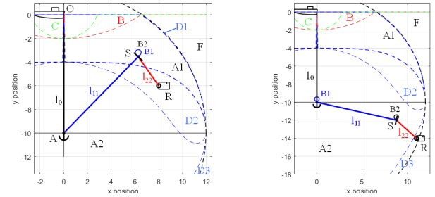
(c) Case l_0 < l_2 + l_1 + h_{b2} , l_1 = 3l_2 (d) Case l_0 < l_2 + l_1 + h_{b2} , l_1 = 3l_2 and F_{b2} = 3F_{b1} . Area D2: buoy B1 and B2 are in contact with the stop, i.e. l_{11} = l_1 , l_{12} = 0 , l_{21} = 0 , l_{22} = l_2 . Area D3: buoy B1 is in contact with the stop, i.e. l_{11} = 0 , l_{12} = 0 , l_{21} = 0 , l_{22} = l_2 .
