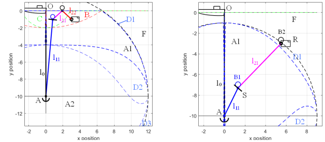
(e) Case l_0 < l_2 + l_1 + h_{b2} , l_1 = 3l_2 (f) Case l_0 > l_2 + l_1 + h_{b2} , l_2 = 2l_1 and F_{b2} = 3F_{b1} . Area B: buoy B1 is in contact with the stop and B2 with the surface, i.e. l_{11} = 0 , l_{12} = l_1 , l_{21} = l_2 , l_{22} = 0 . Area D1: buoy B1 is in contact with the stop and B2 the surface, i.e. l_{11} = 0 , l_{12} = l_1 , l_{21} = 0 , l_{22} = 0 .
