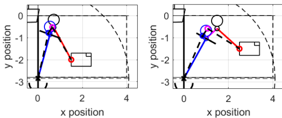
(a) Left: E_{B2} = 0.098m . Right: E_{B2} = 0.434m
