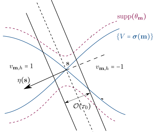
FIGURE 4.2. The support of the function v_{\mathbf{m},h}
