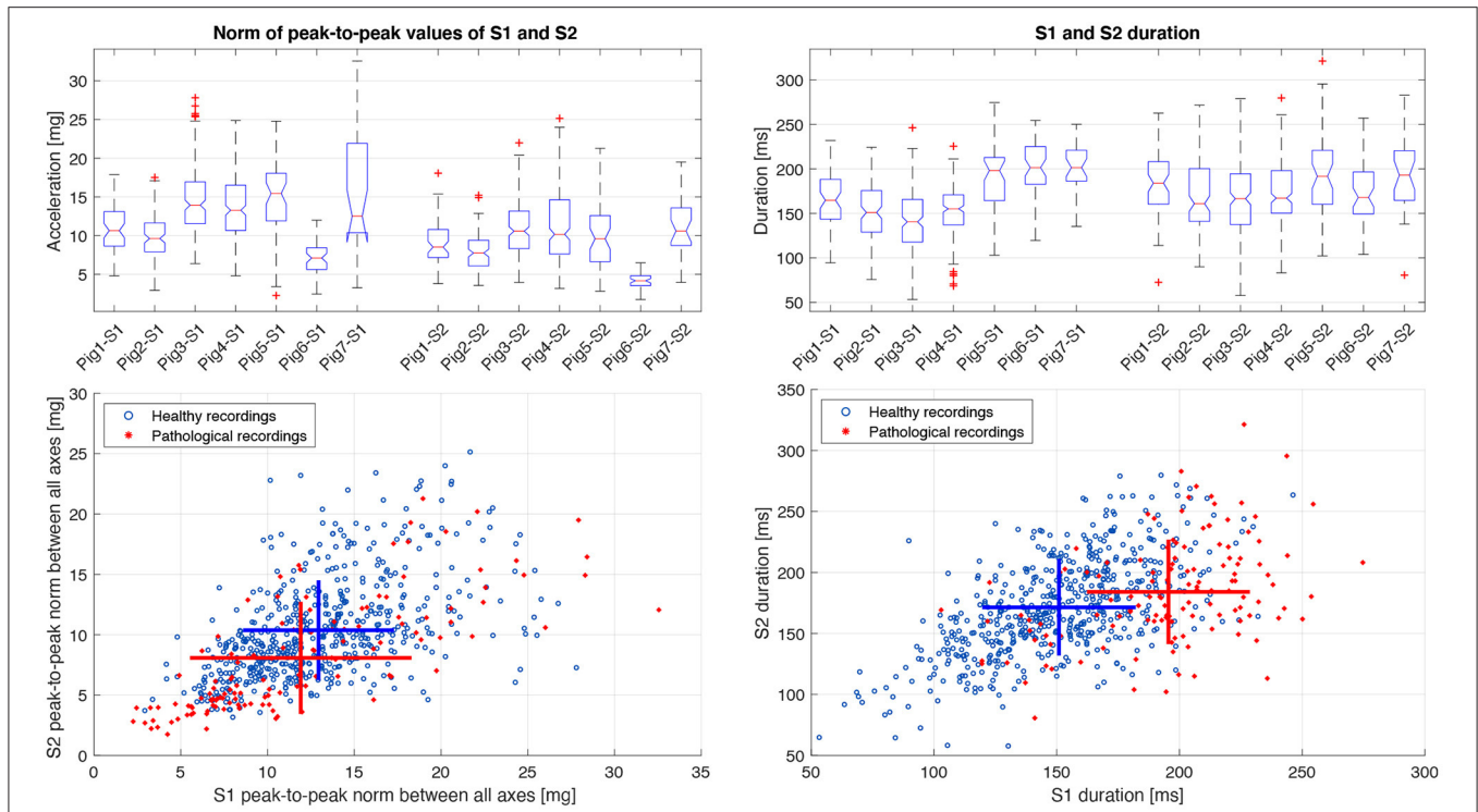
FIGURE 10 | Statistical distribution and scatter plot of the norm of the peak-to-peak values between all ACC axes and the duration of S1 and S2 between healthy and pathological pigs. The crosses in the scatter plot represent the mean and standard deviation of each population.
