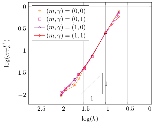
Figure 2: Convergence order
