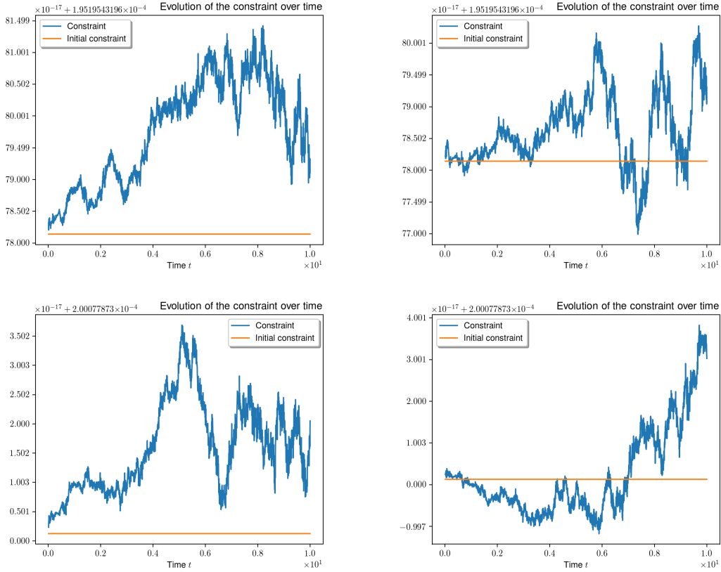
Figure 3: Evolution of the constraint in time for several couples (\mathbf{m}, \gamma) : (0, 0) upper left, (0, 1) upper right, (1, 0) bottom left, (1, 1) bottom right. The initial constraint is non zero and is represented by the orange horizontal line.
