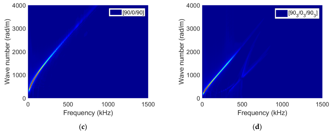
Figure 12. Simulated dispersion curves (wavenumber k as a function of frequency f ) using 2D-FFT of signals recorded along a straight line perpendicular to the crack surface on the specimen top surface for a) [0/90/0], b) [0 3 /90 3 /0 3 ], c) [90/0/90] and d) [90 3 /0 3 /90 3 ] specimens.
