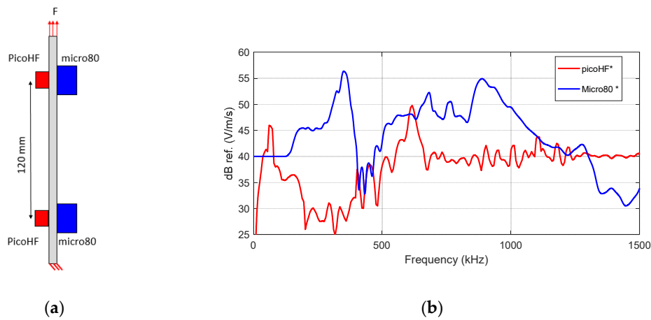
Figure 1. (a) Location of the sensors on the specimen (b) Frequency sensitivity functions of picoHF and micro80 sensors used to capture acoustic emission during tensile tests in composite laminates (calibration curve obtained on steel block with reciprocity method).
