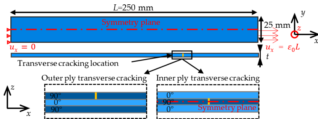
Figure 2. Dimensions of the modeled specimens. Transverse cracking occurs in a 90 deg. Ply with respect to the loading direction.
