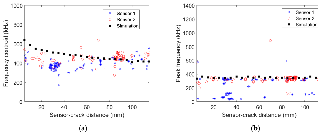
Figure 8. (a) Frequency centroid (b) peak frequency as a function of the distance between the AE source and the micro80 sensors obtained experimentally for the [0/90/0] specimen and numerically.
