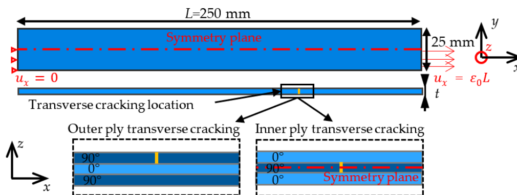
Figure 2. Dimensions of the modeled specimens. Transverse cracking occurs in a 90 deg. Ply with respect to the loading direction.
