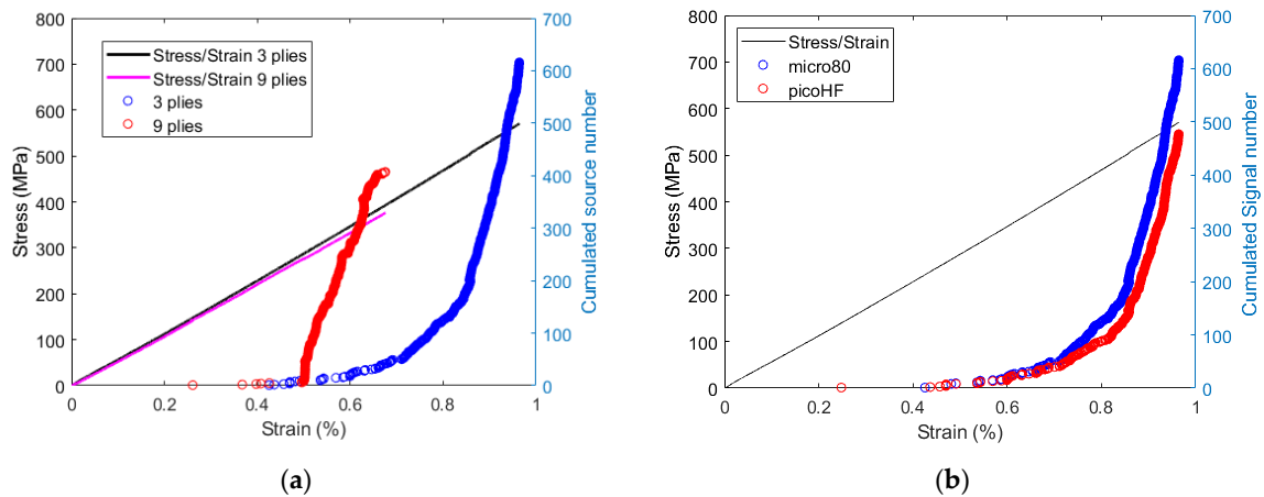
Figure 4. Cumulated localized signal number and stress as a function of strain for (a) [0/90/0] and [0 3 /90 3 /0 3 ] specimens using the micro80 sensor and (b) micro80 and picoHF sensors for [0/90/0] specimens.
