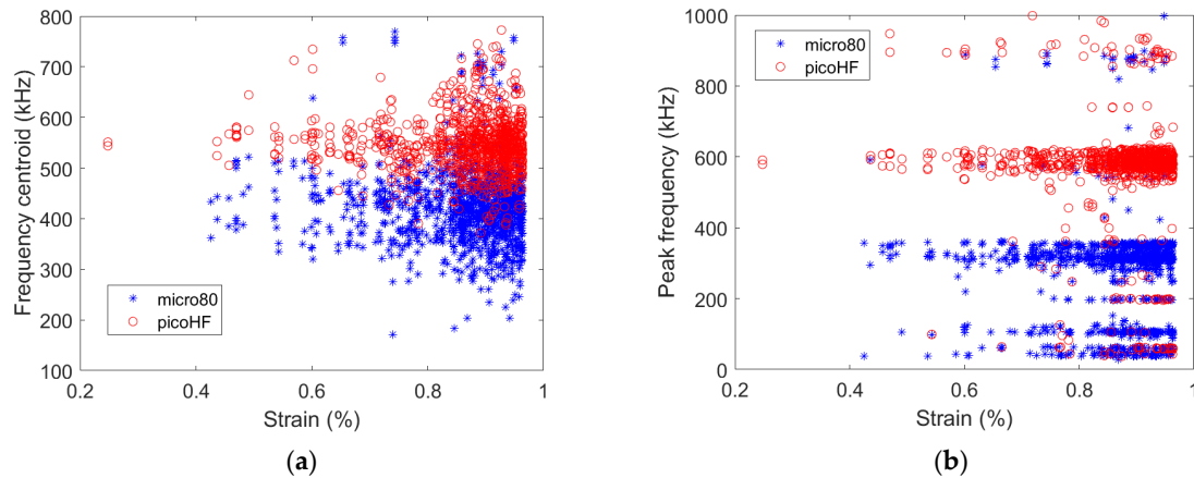
Figure 5. (a) Frequency centroid and (b) peak frequency as a function of strain obtained for the [0/90/0] specimen (thickness = 0.9 mm) with either micro80 or picoHF sensors.
