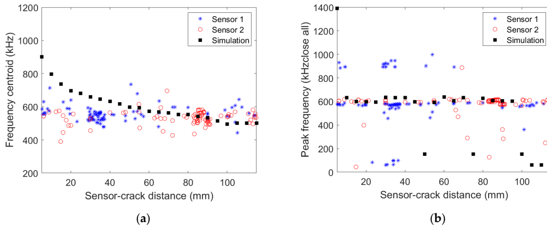
Figure 9. (a) Frequency centroid (b) peak frequency as a function distance between the AE source and the picoHF sensors obtained experimentally for the [0/90/0] specimen and numerically.
