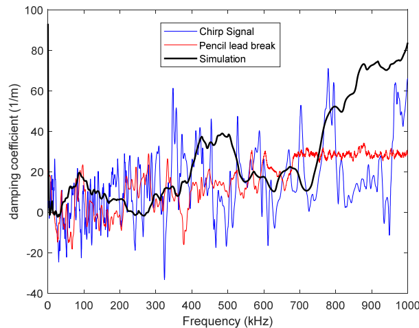
Figure 3. Damping coefficient as a function of the frequency obtained experimentally for (i) emitted chirp and (ii) pencil lead break and (iii) numerically.
