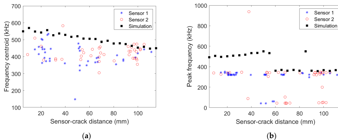
Figure 7. (a) Frequency centroid and (b) peak frequency as a function of the distance between the AE source and the micro80 sensors obtained experimentally for the [0 3 /90 3 /0 3 ] specimen and numerically.
