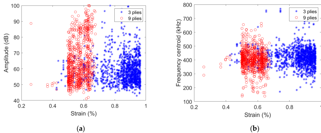
Figure 6. (a) Amplitude and (b) frequency centroid as a function of strain obtained with micro80 sensor for [0/90/0] or [0 3 /90 3 /0 3 ] specimens.
