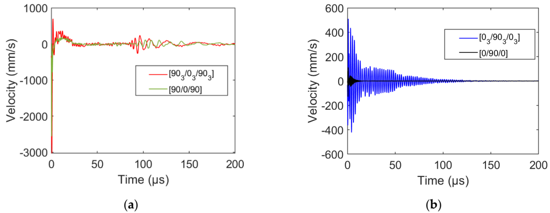
Figure 10. Out-of-plane velocity as a function of time obtained at crack epicenter for (a) outer ply transverse cracking in [90_n/0_n/90_n] specimens and (b) inner ply transverse cracking in [0_n/90_n/0_n] , ( n = 1 or 3 ).
