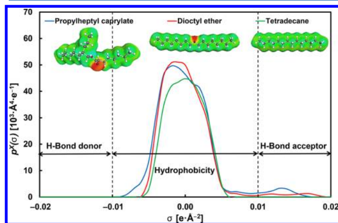
Figure 2. Plots of \sigma -surfaces and \sigma -profiles of three cosmetic oils: propylheptyl caprylate (blue), dioctyl ether (red), and tetradecane (green) using the COSMO-RS model.
