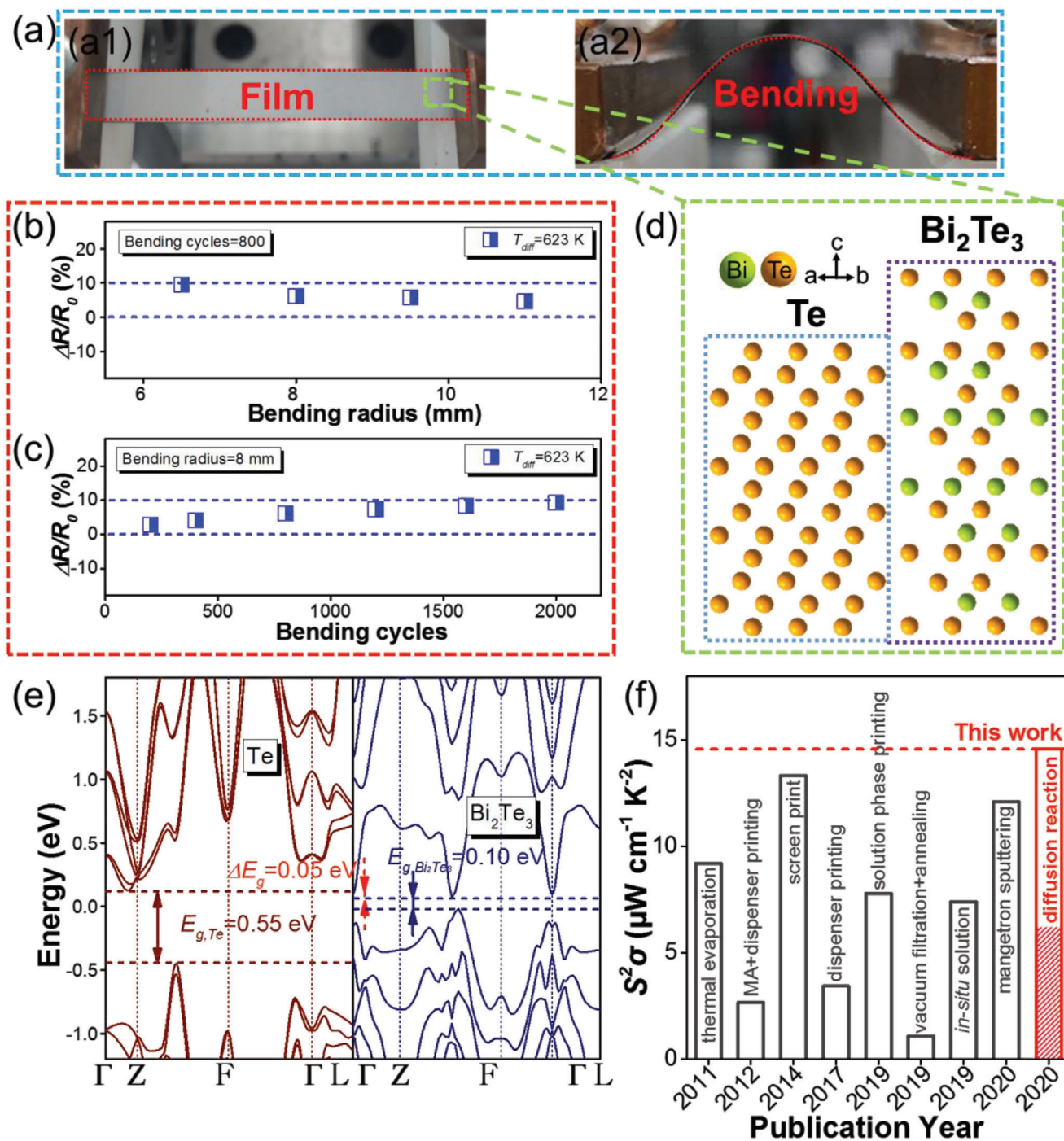
Figure 1. a) Optical images of as-prepared Bi 2 Te 3 flexible thin film under (a1) flat and (a2) bending statuses, respectively. b) The \Delta R/R_0 of the Bi 2 Te 3 flexible thin film prepared under the diffusion temperature of 623 K as a function of bending radius at the bending cycles of 800 times. c) The \Delta R/R_0 of the Bi 2 Te 3 flexible thin film prepared under the diffusion temperature of 623 K as a function bending cycles at the bending radius of 8 mm. d) Schematic structure of Bi 2 Te 3 and Te. e) DFT calculated electronic band structures of Te and Bi 2 Te 3 , respectively. f) Comparison of the maximum room-temperature S^2\sigma between our Bi 2 Te 3 -based flexible thin films and other state-of-art n-type Bi 2 Te 3 -based flexible thin films prepared by different methods, including thermal evaporation (2011), [35] mechanically alloyed (MA) and dispenser printing (2012), [19] screen print (2014), [34] dispenser printing (2017), [32] solution phase printing (2019), [30] vacuum filtration and annealing (2019), [31] in situ solution (2019), [33] magnetron sputtering (2020), [36] and this work.
