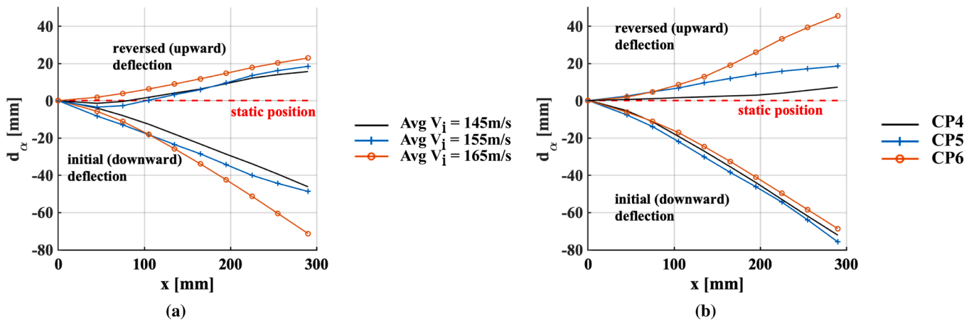
Fig. 19. Variation in the \alpha - axis displacement of each point LE1 - LE8 showing a side-on profile view of the minimum and maximum displacements across all points in time; (a) shows average results observed at each distinct test speed and (b) shows results for each test (CP4 - CP6) at the ultimate test velocity V_i = 165\text{m/s} .
