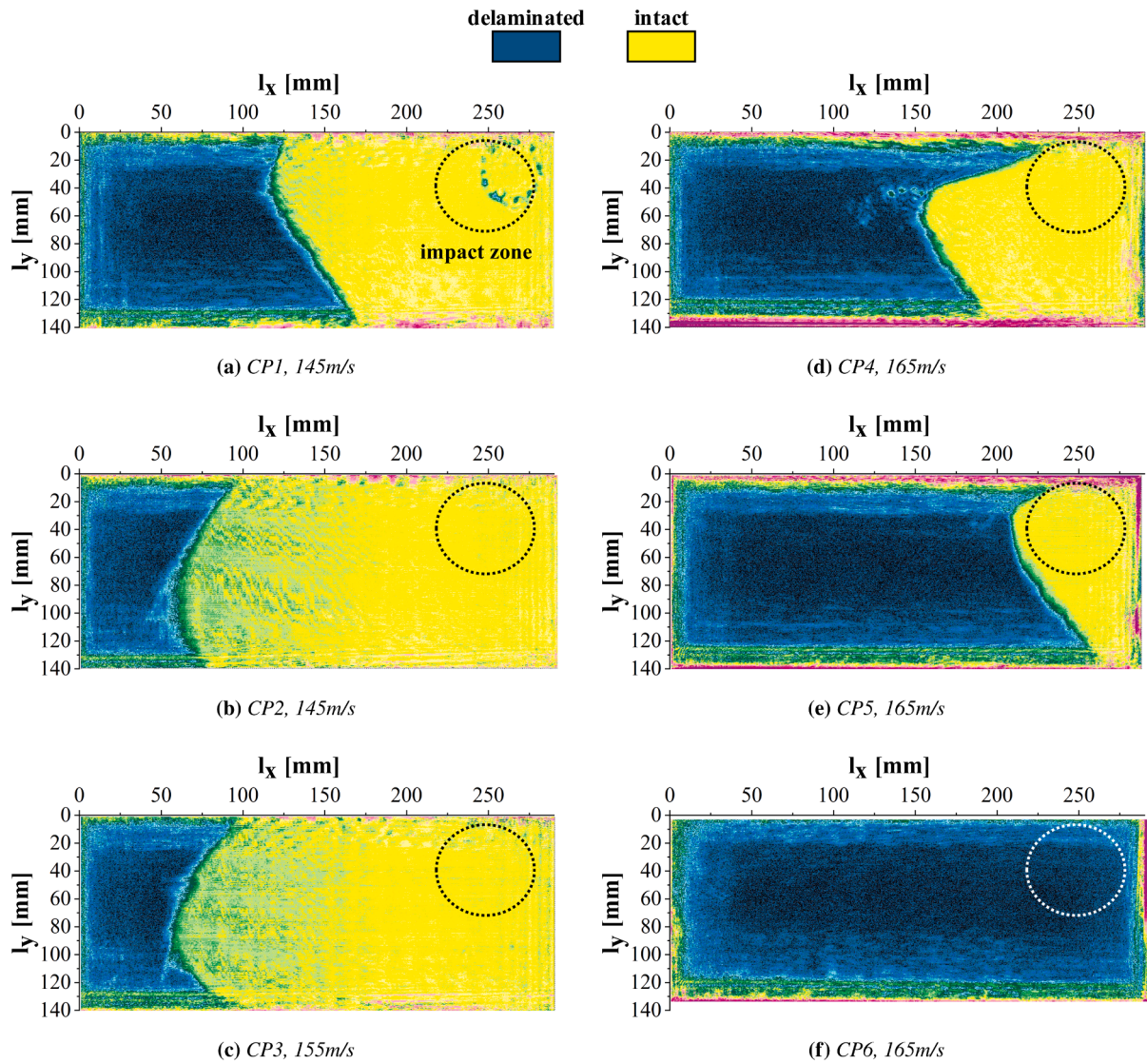
Fig. 23. C-scan plots of delamination for unpinned laminates CP1 - CP6, showing region of impact. The specimen root corresponds to l_x = 0\text{mm} , the visible edge in HSV1 corresponds to l_x = 290\text{mm} and the visible edge in HSV2 corresponds to l_y = 140\text{mm} .
