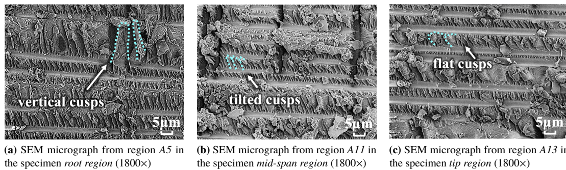
Figure 28: Illustration of the variation in cusp out-of-plane tilt with mode-ratio with corresponding SEM micrographs taken from the upper surface in Figure 27 - a) Near root, b) mid-length and c) near tip
