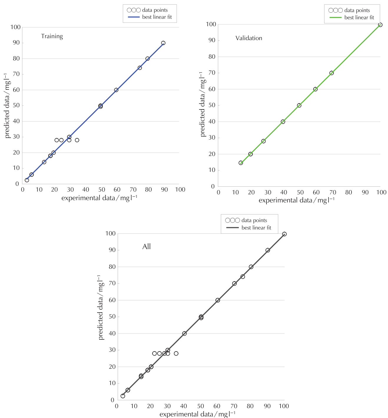
Fig. 6 – Relation between the observed dose of coagulant and those estimated by the ANN model
